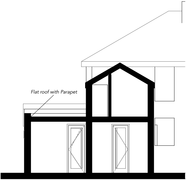
D Proposed Section D 1:100
