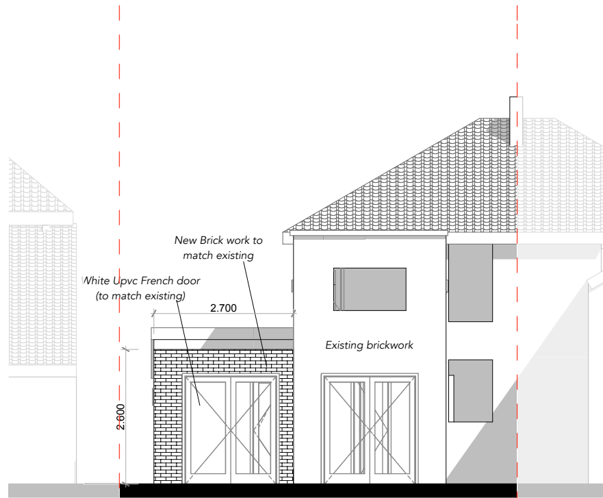
Ai Proposed Front Elevation 1:100
