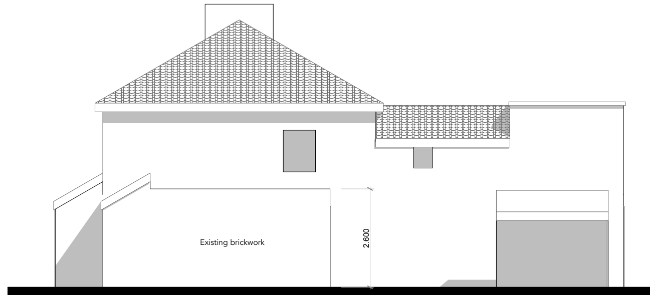
D Side Elevation 1:100
