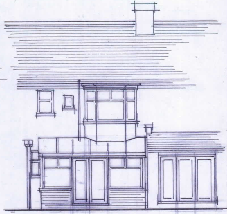
EXIST REAR ELEV
