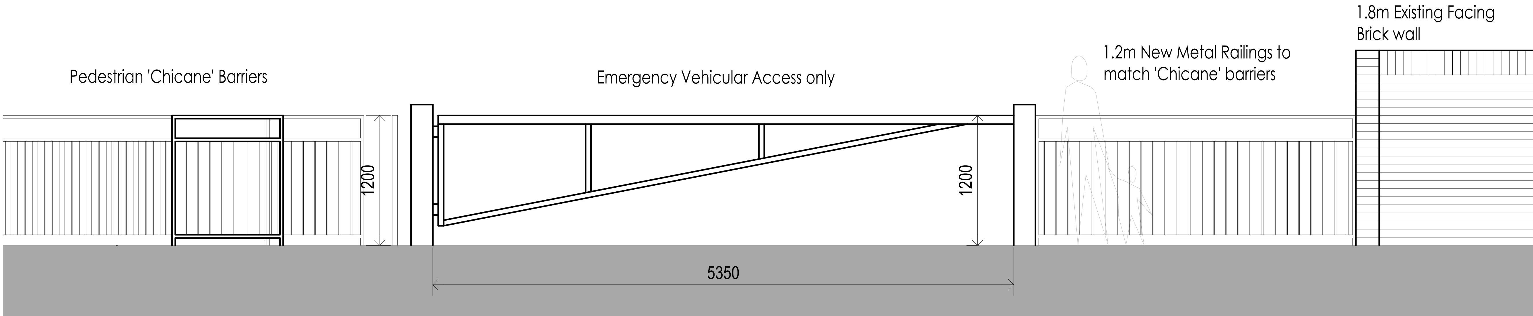
Gate Elevation - Showing Pedestrian & Vehicle Restriction along Chalfont Rd Scale: 1:20 @A1
