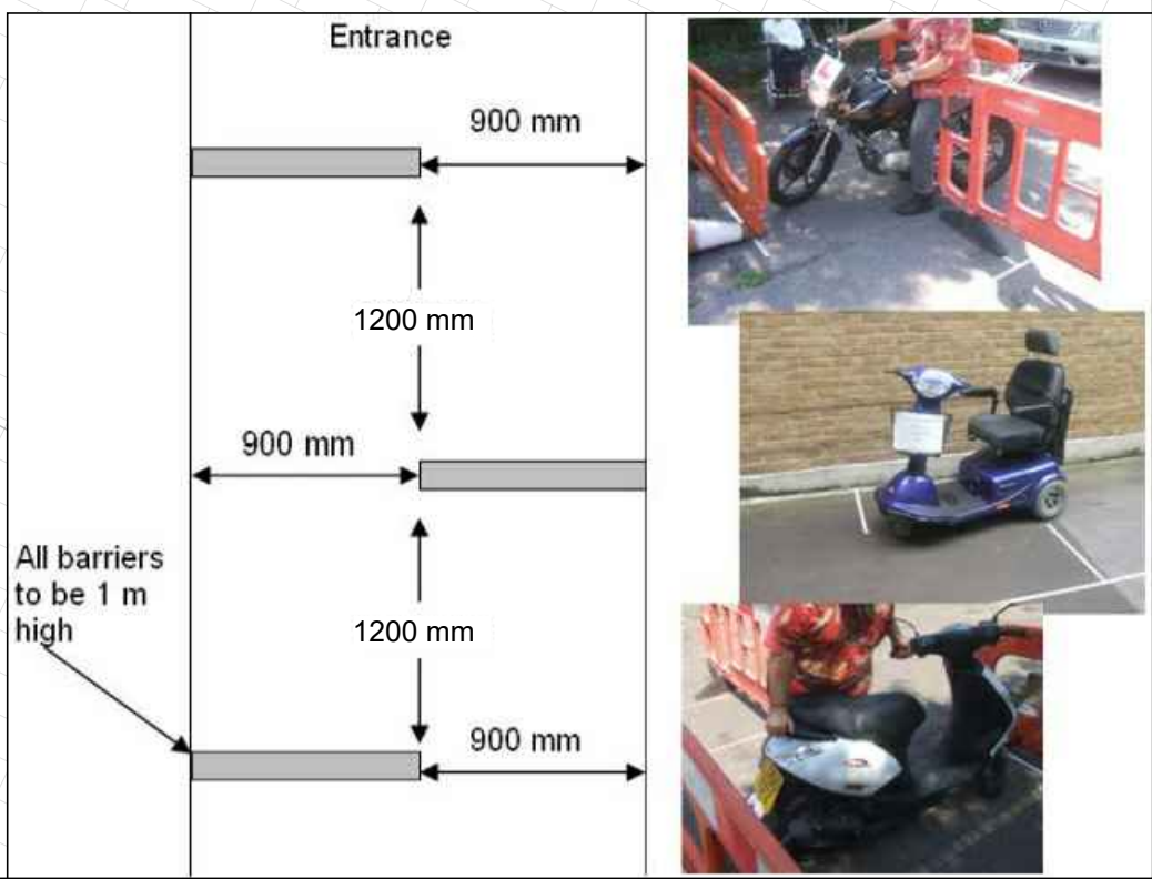
Plan of Chicane Barriers
