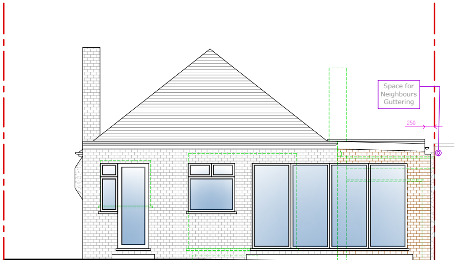
5 Proposed Rear Elevation
