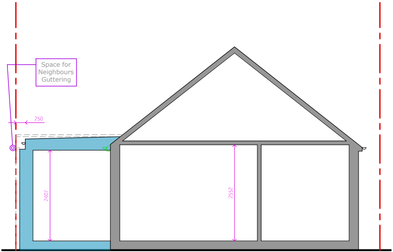
8 Proposed Front Section
