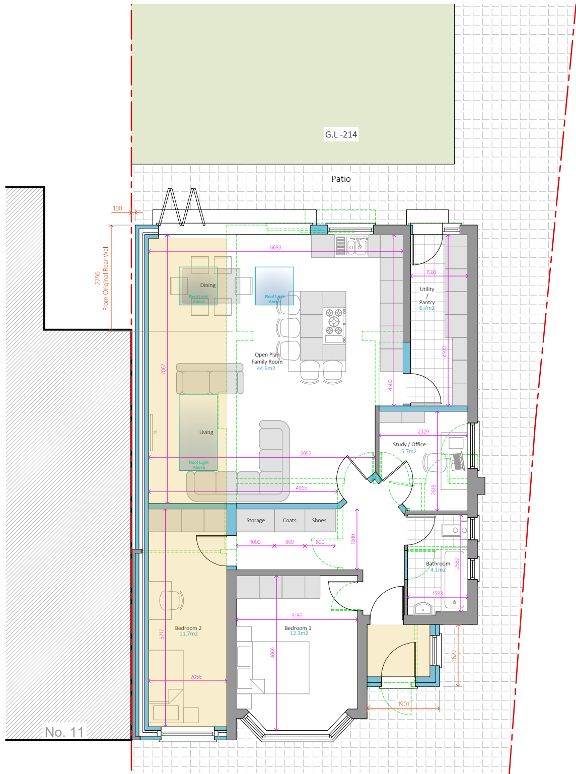
1 Proposed Ground Floor Plan
