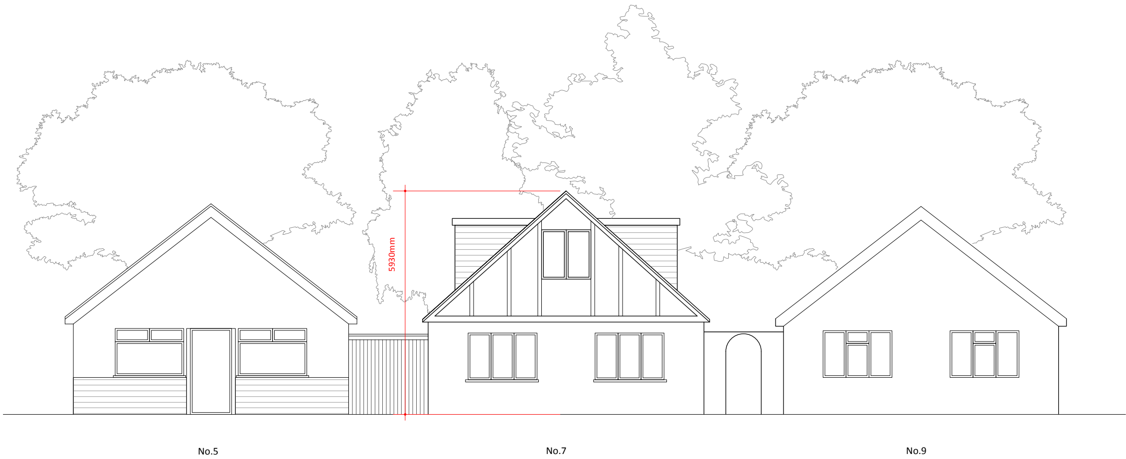
1 ELEVATION A
