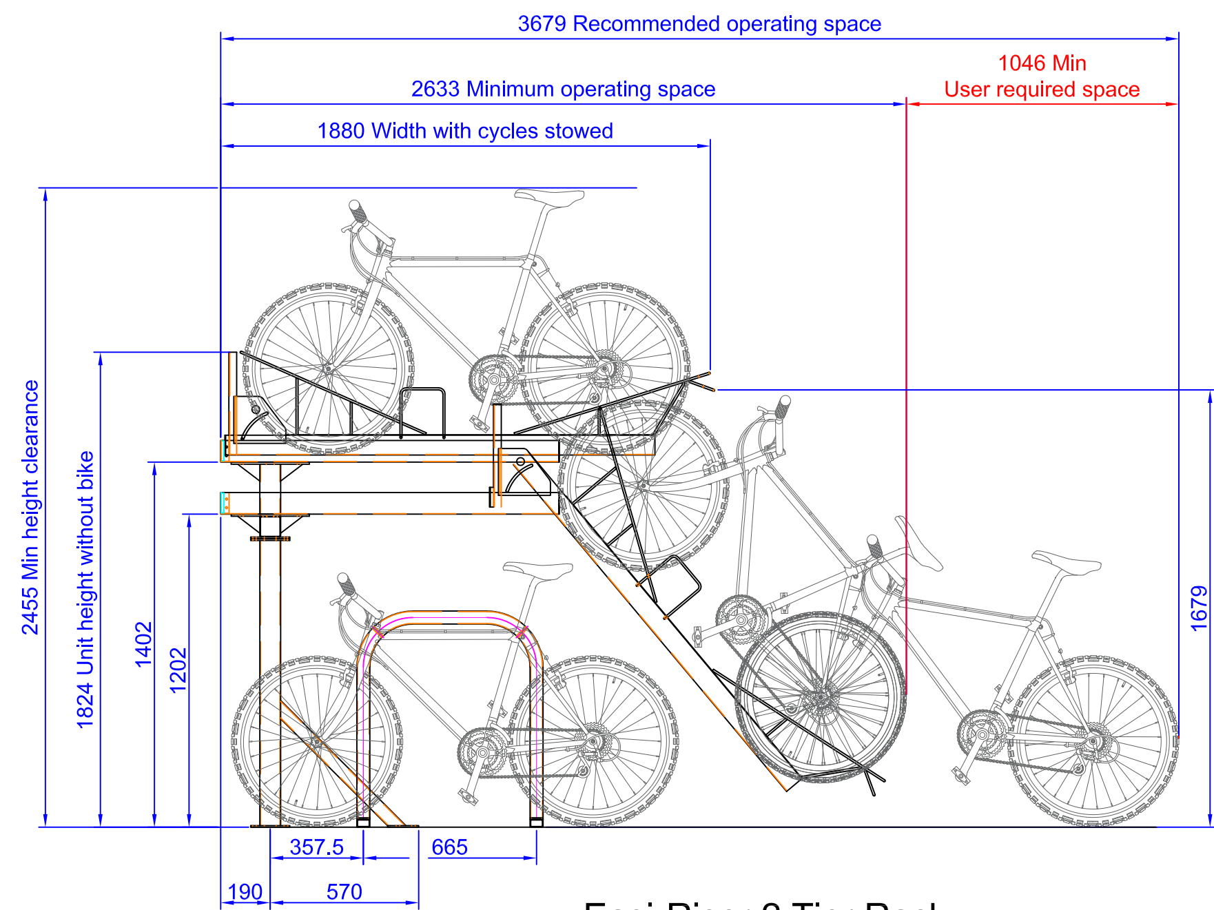
Easi-Riser 2 Tier Rack
