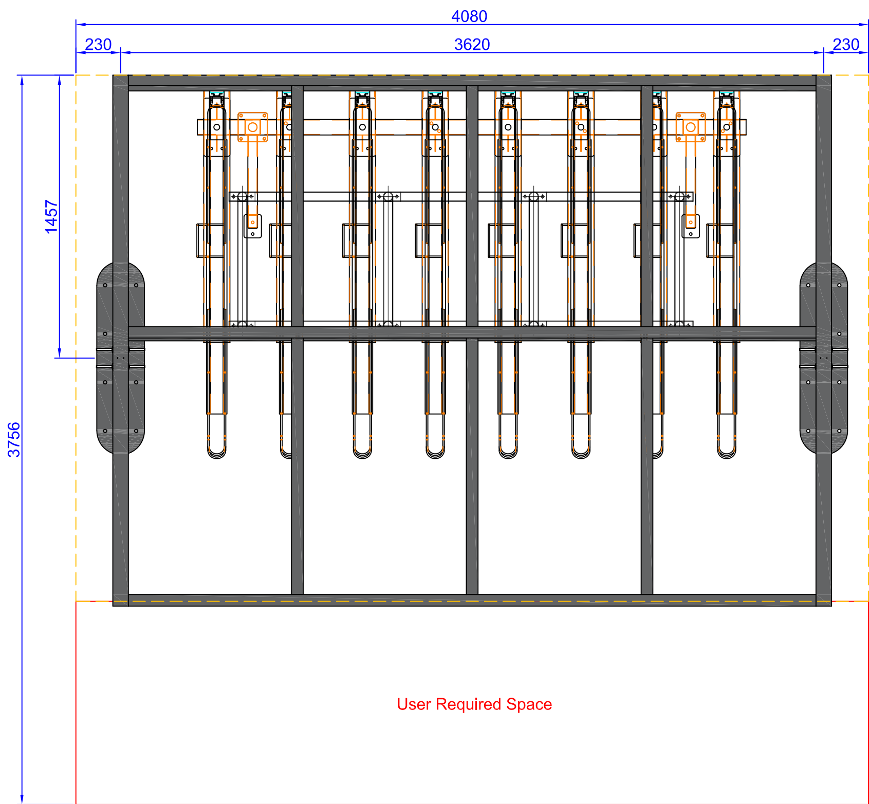
Plan View
