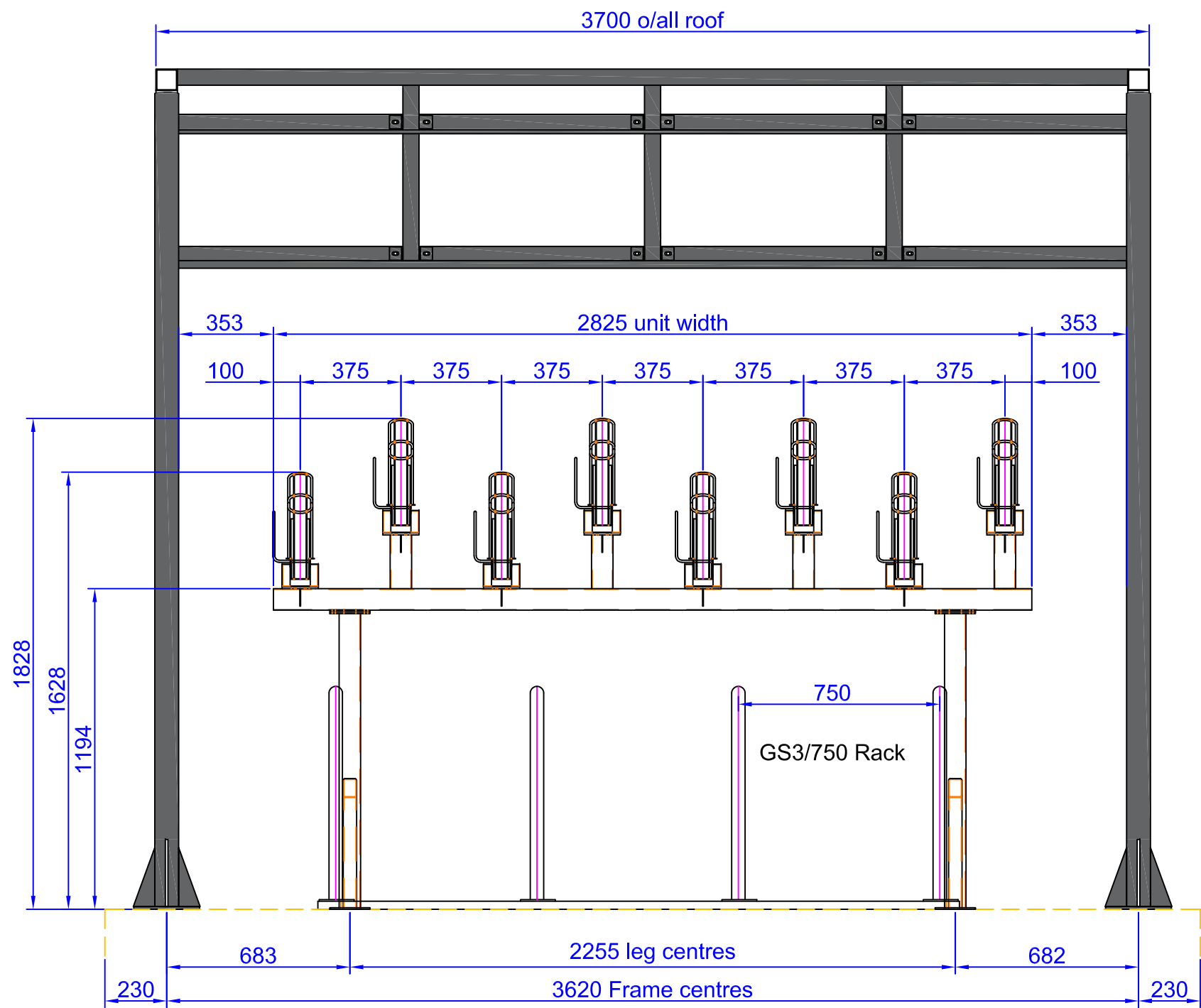
3600 Apollo with Easi-Riser Configuration 8&8
