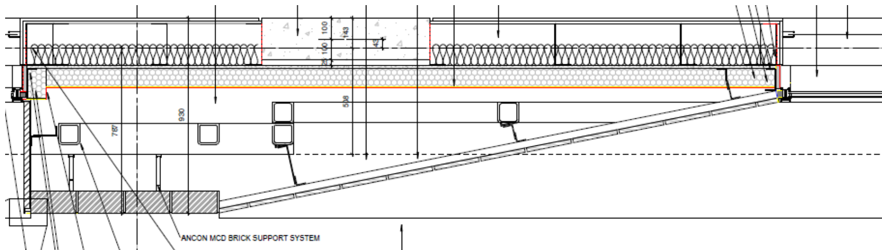
Previous Design with Brick Slips
