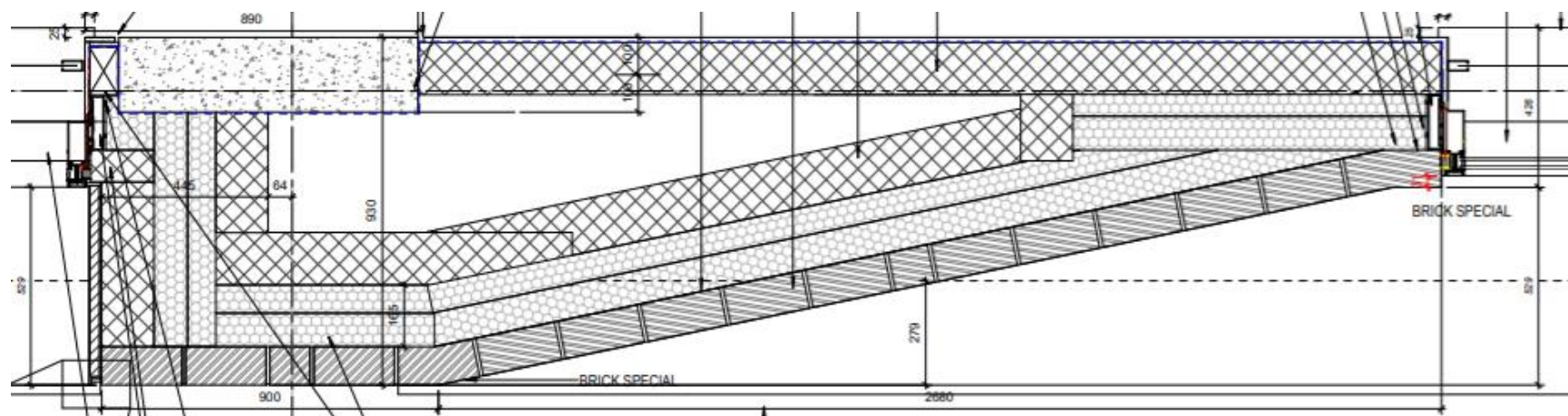
Current Design with Full Sized Bricks
