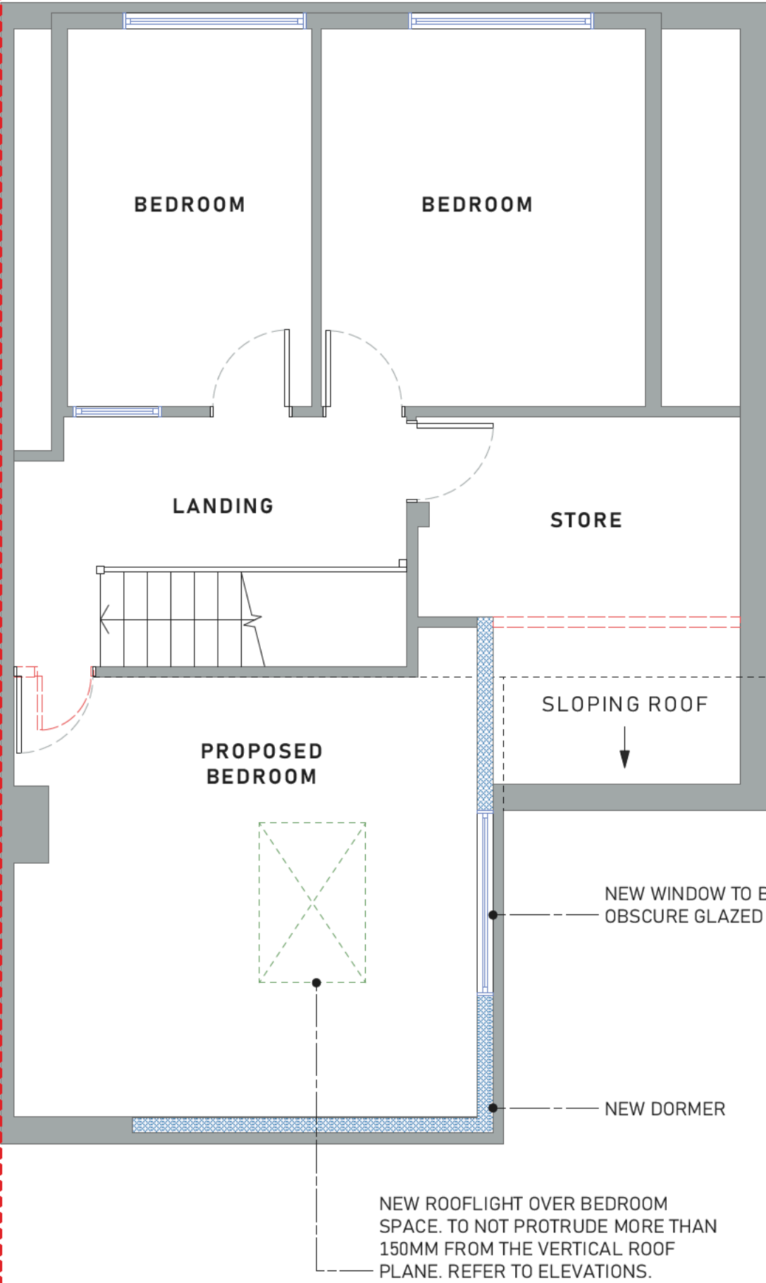
Proposed Loft Floor Scale: 1:50
