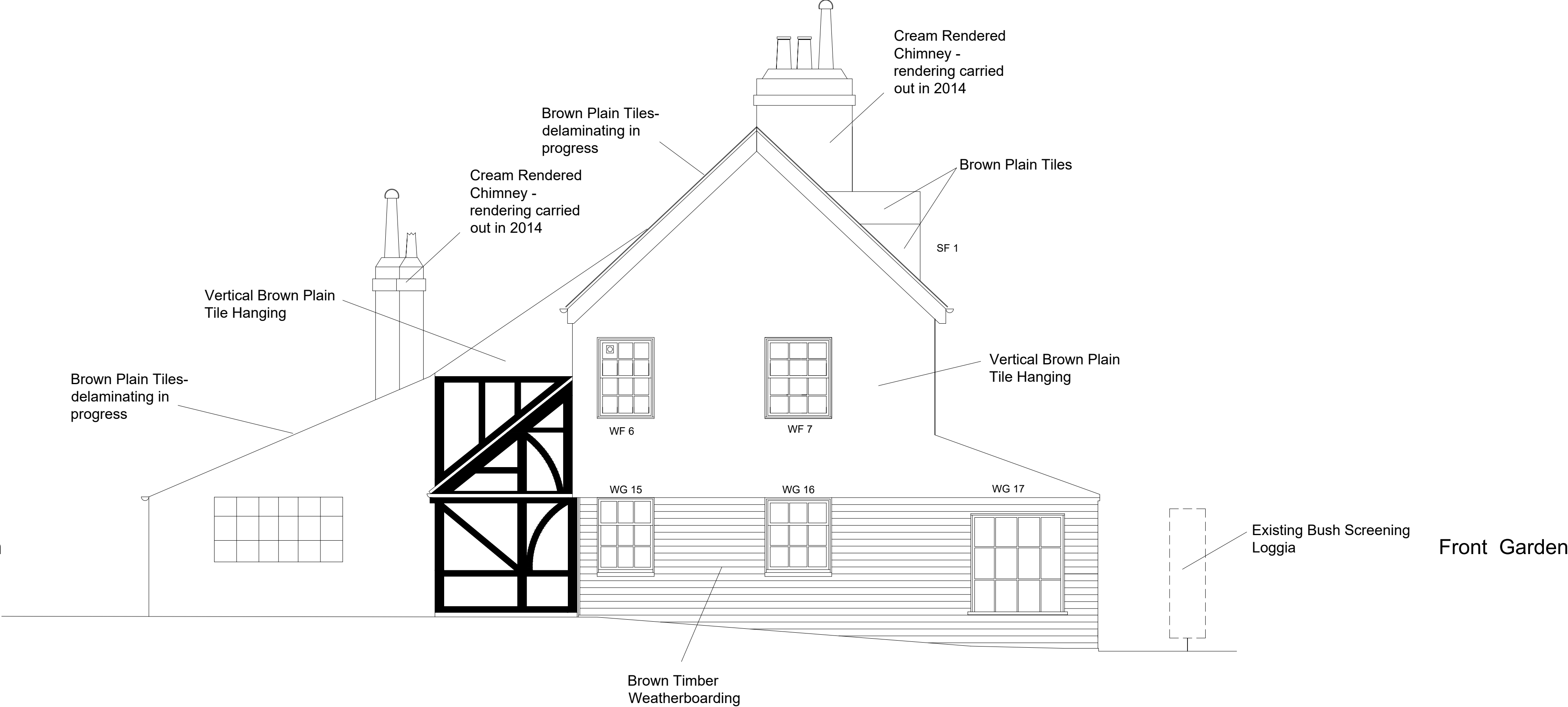
Existing Side Elevation Facing Drive Scale 1:50 @ A1
