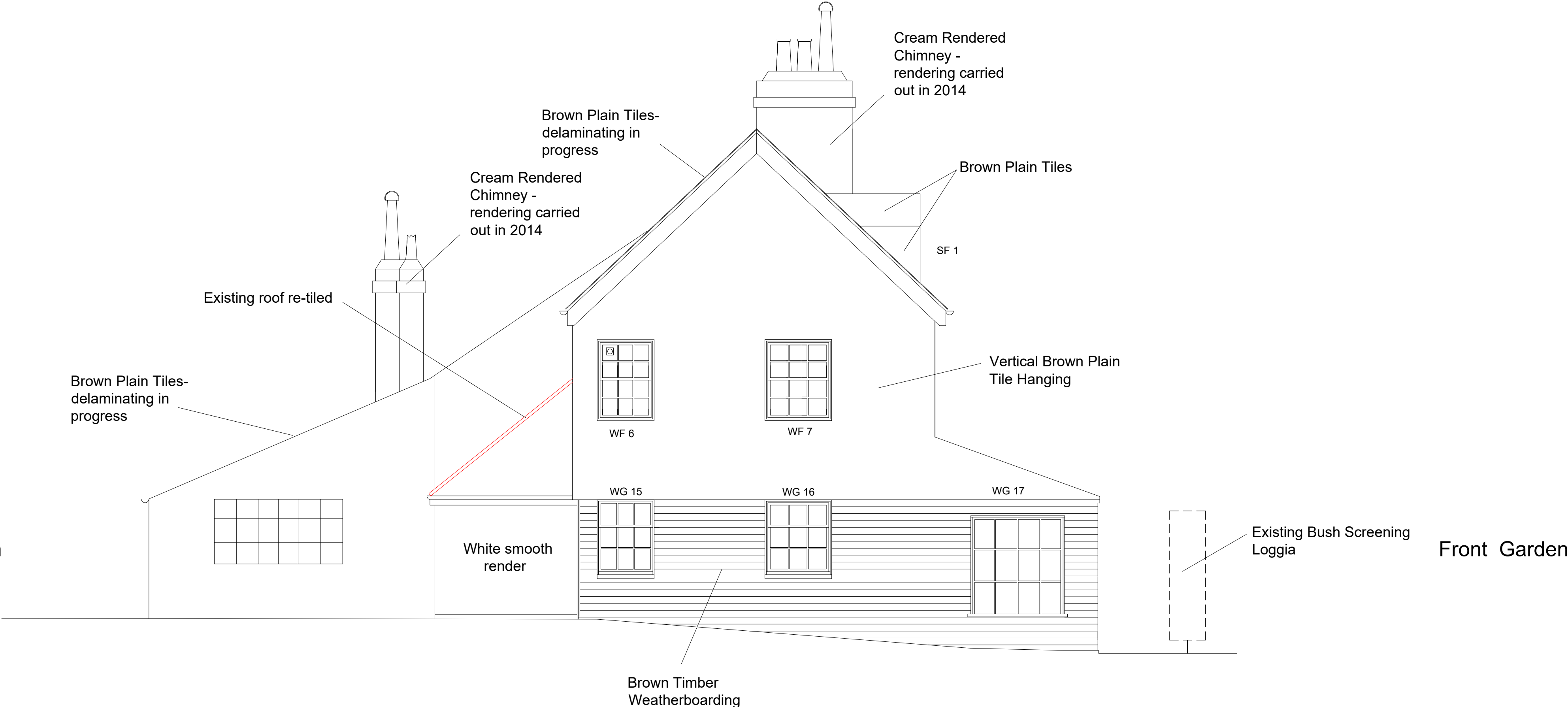
Proposed Side Elevation Facing Drive Scale 1:50 @ A1
