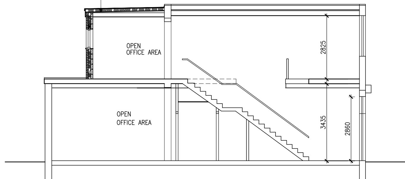
SECTION AA PROPOSED
