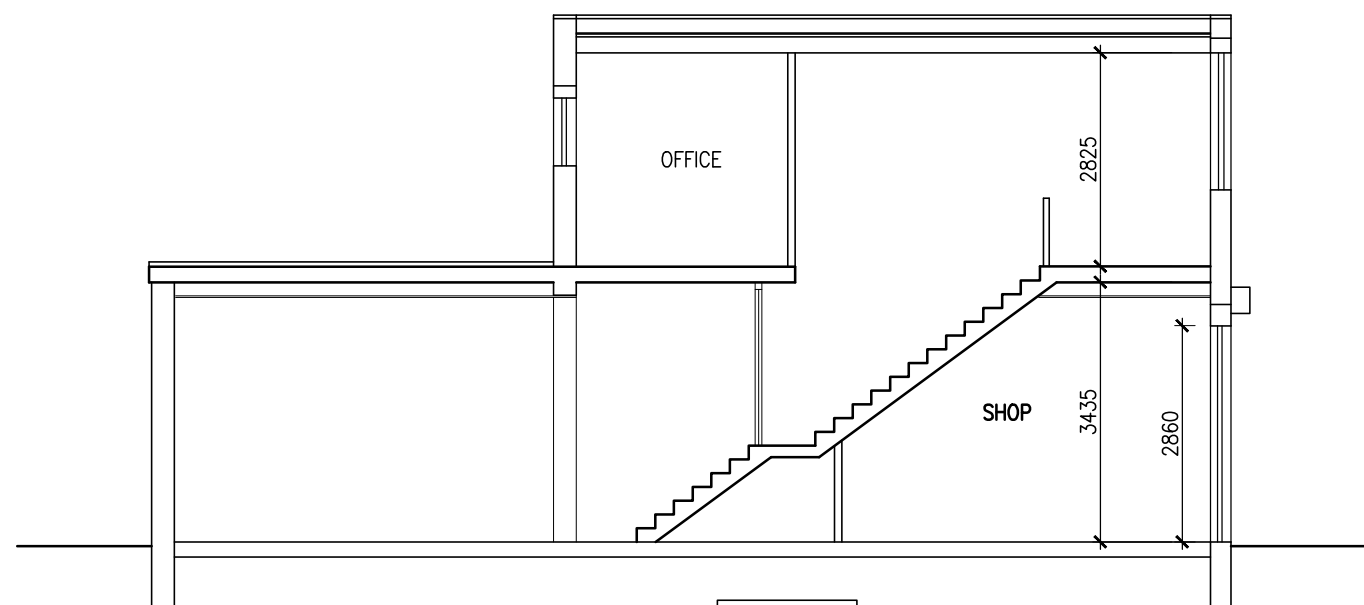
SECTION AA EXISTING
