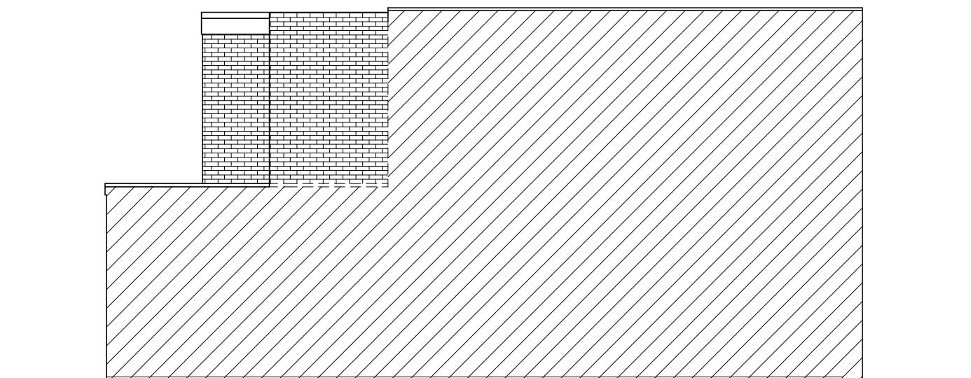
SIDE ELEVATION (THROUGH PARTY WALL)
