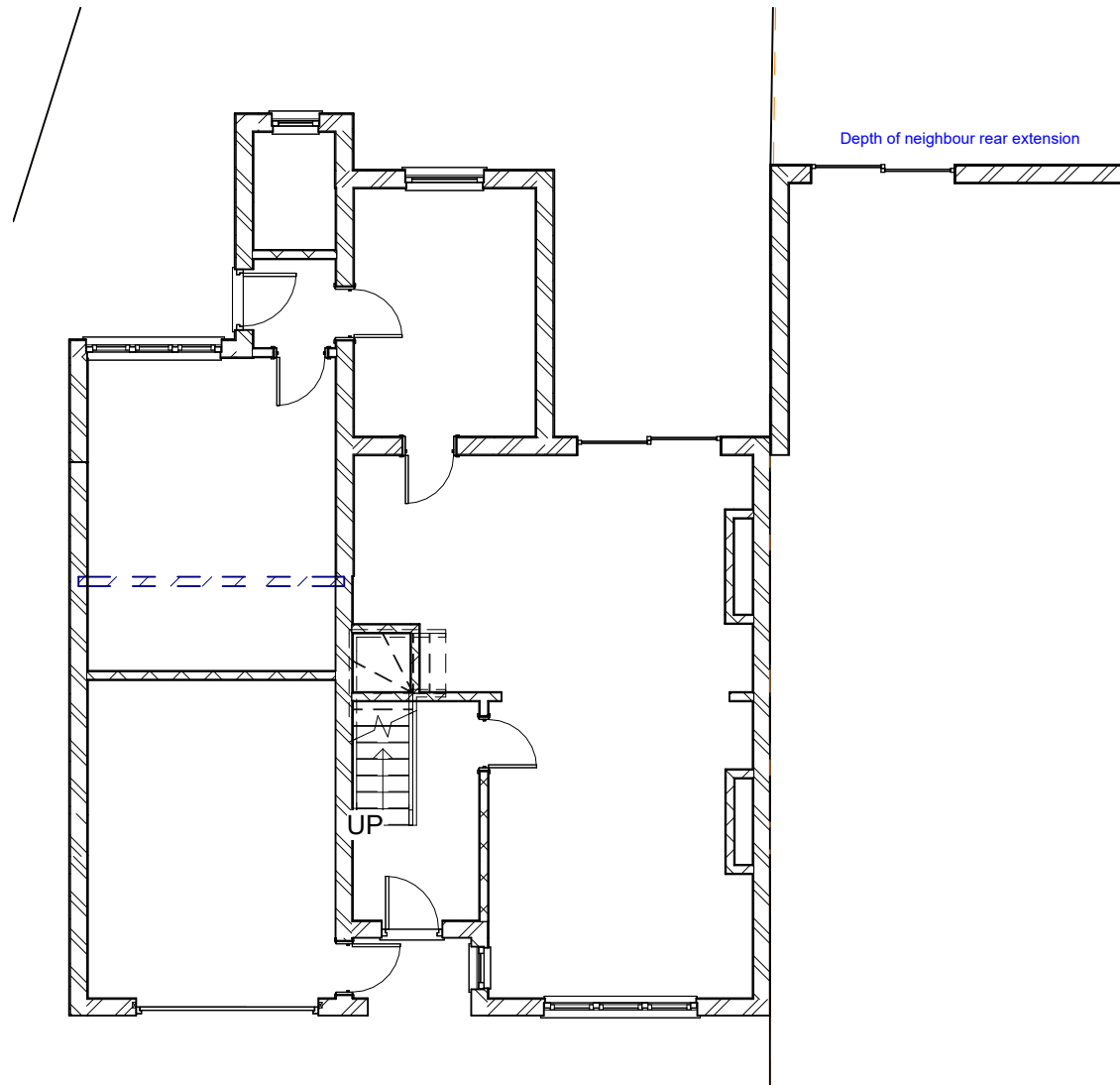
2 Ground Floor 1 : 100
