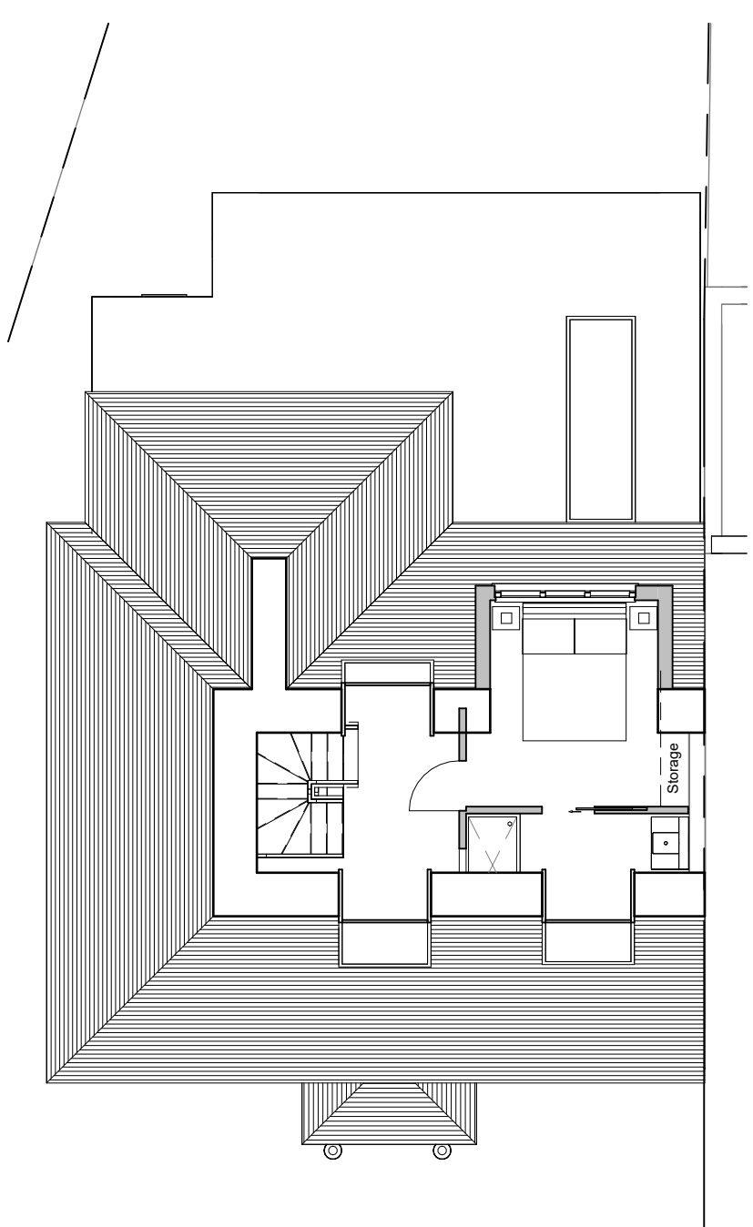
8 Second Floor 1:100
