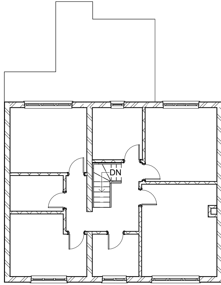
3 First Floor 1 : 100
