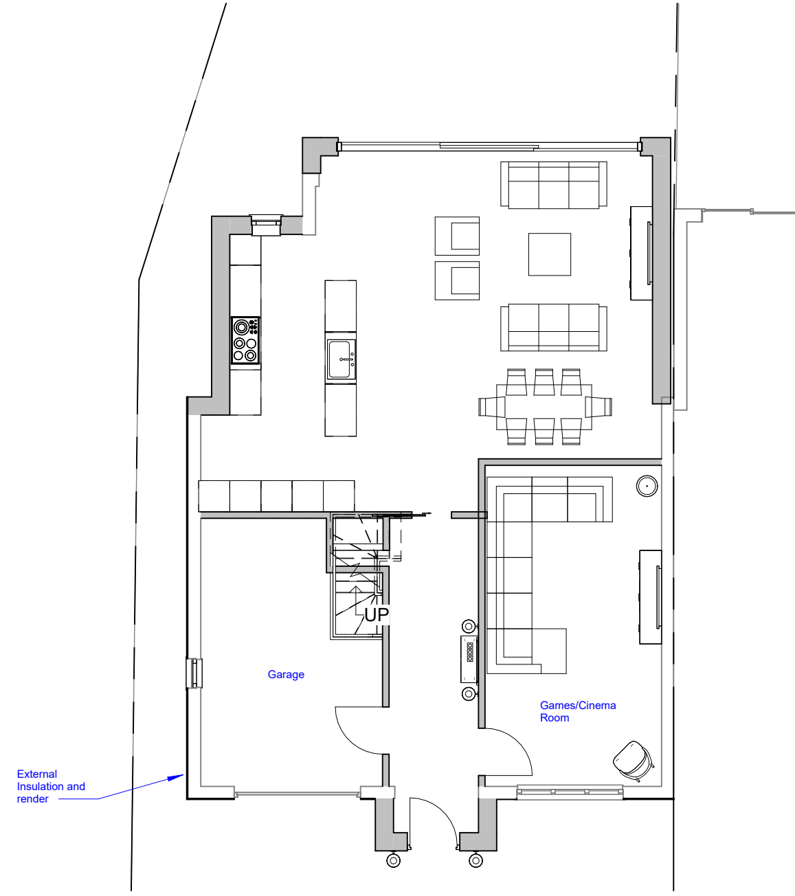
2 Ground Floor 1:100
