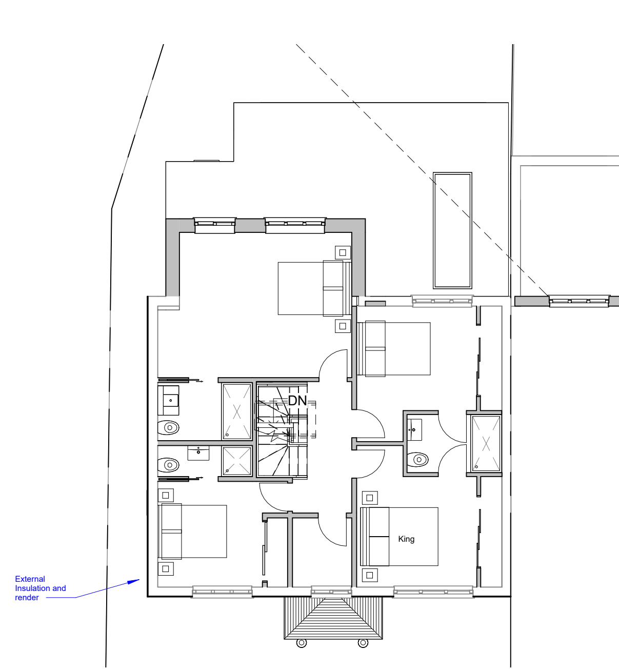
3 First Floor 1:100
