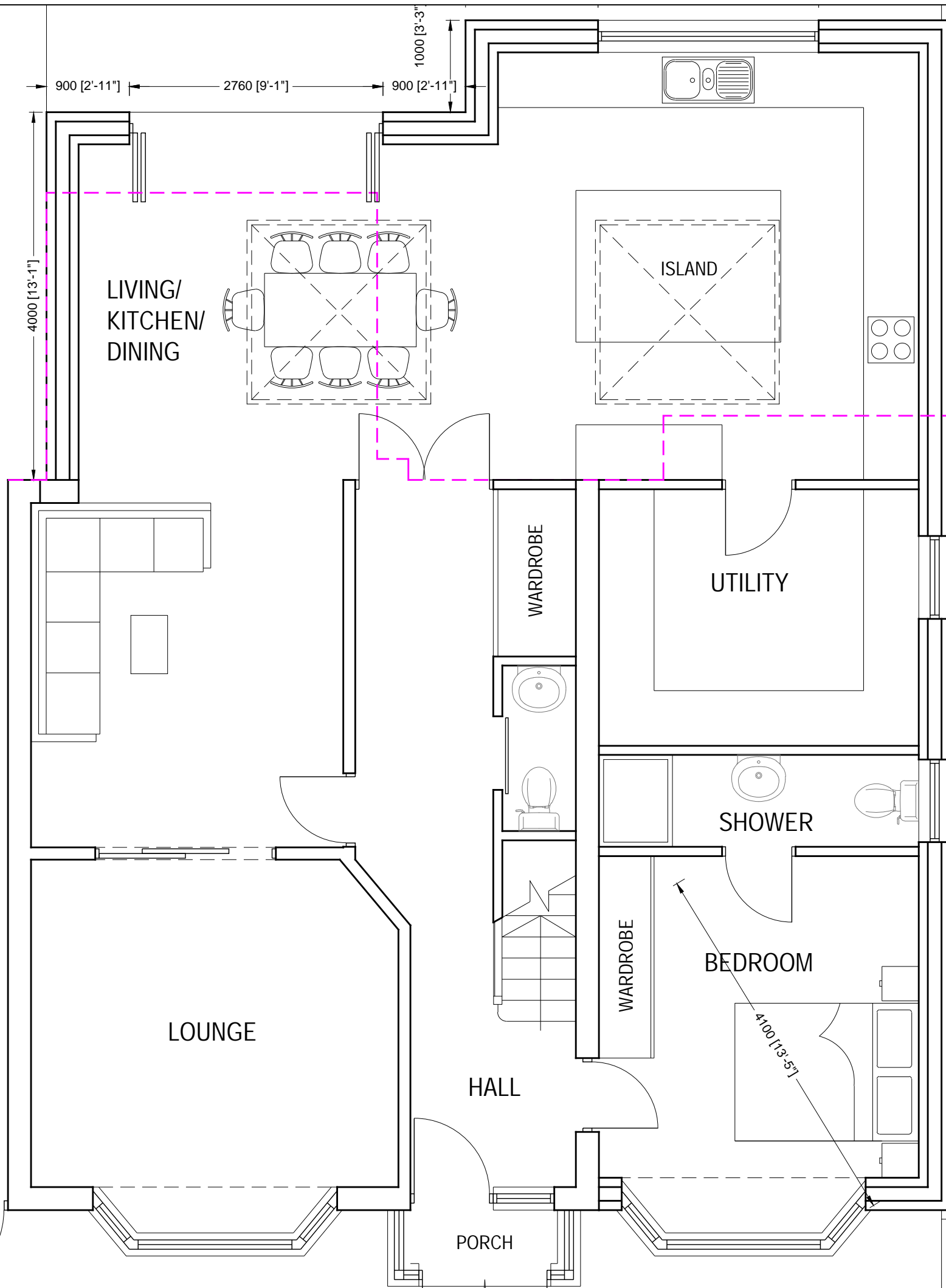
PROPOSED GROUND FLOOR PLAN SCALE-1:500
