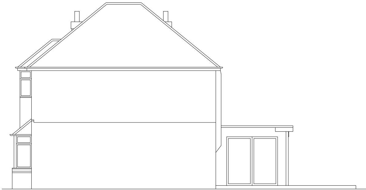
EXISTING ANOTHER SIDE ELEVATION
