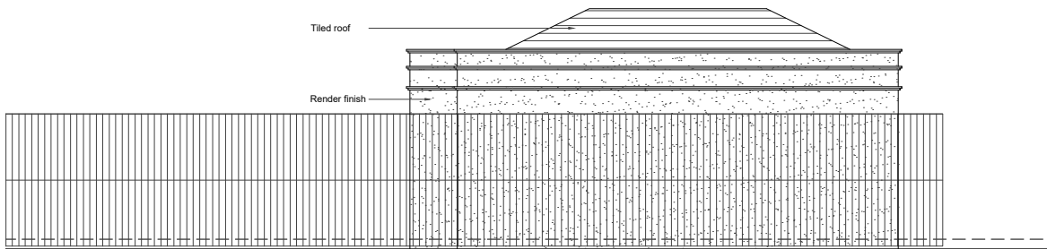
06 - RIGHT SIDE ELEVATION
