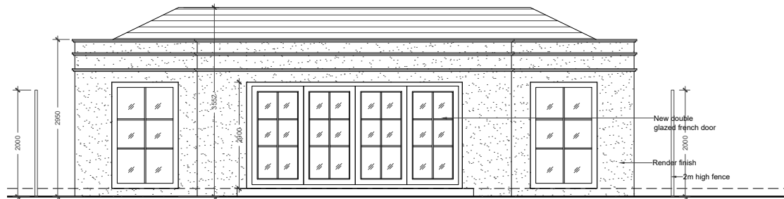
03 - FRONT ELEVATION
