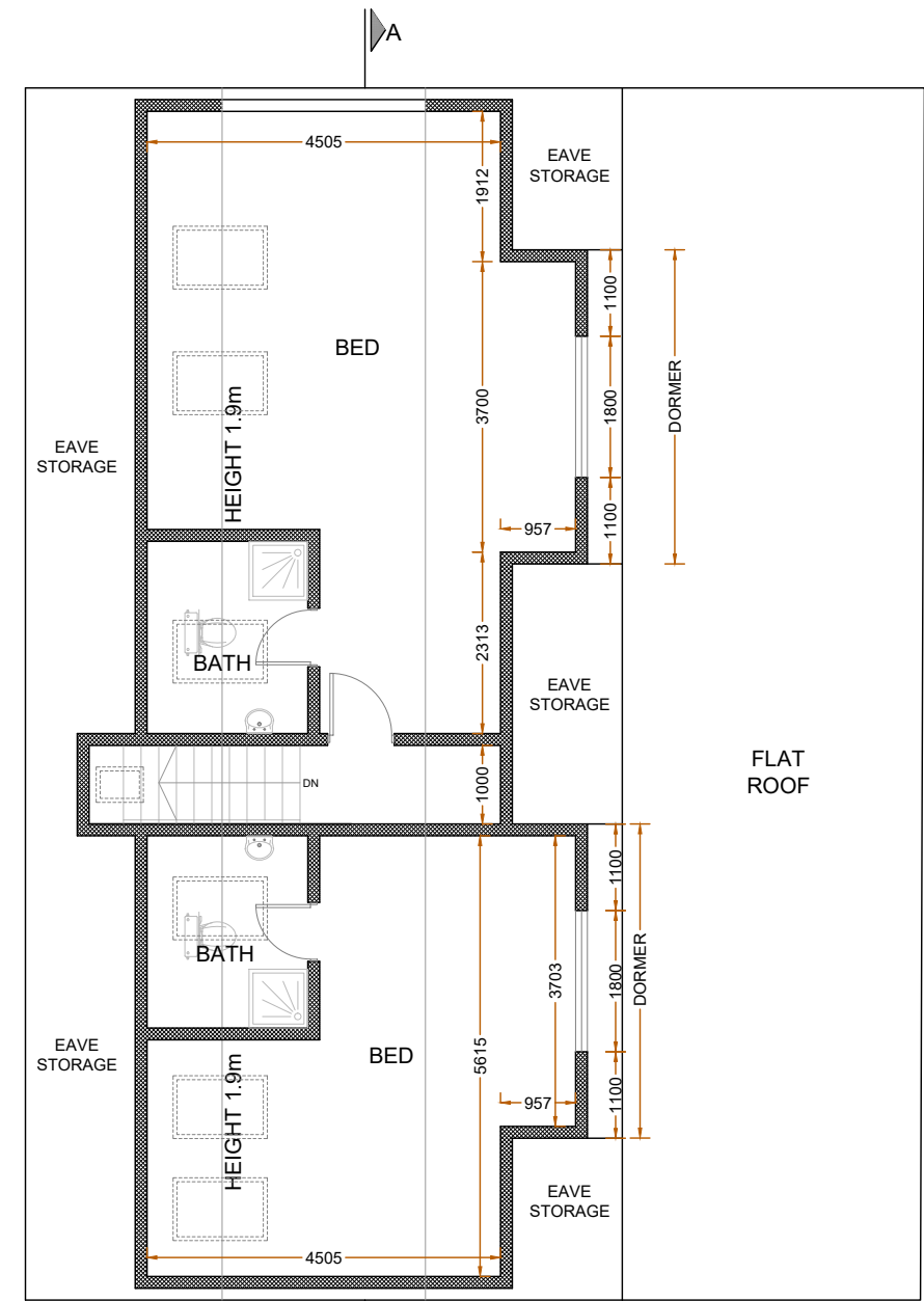
PROPOSED LOFT PLAN
