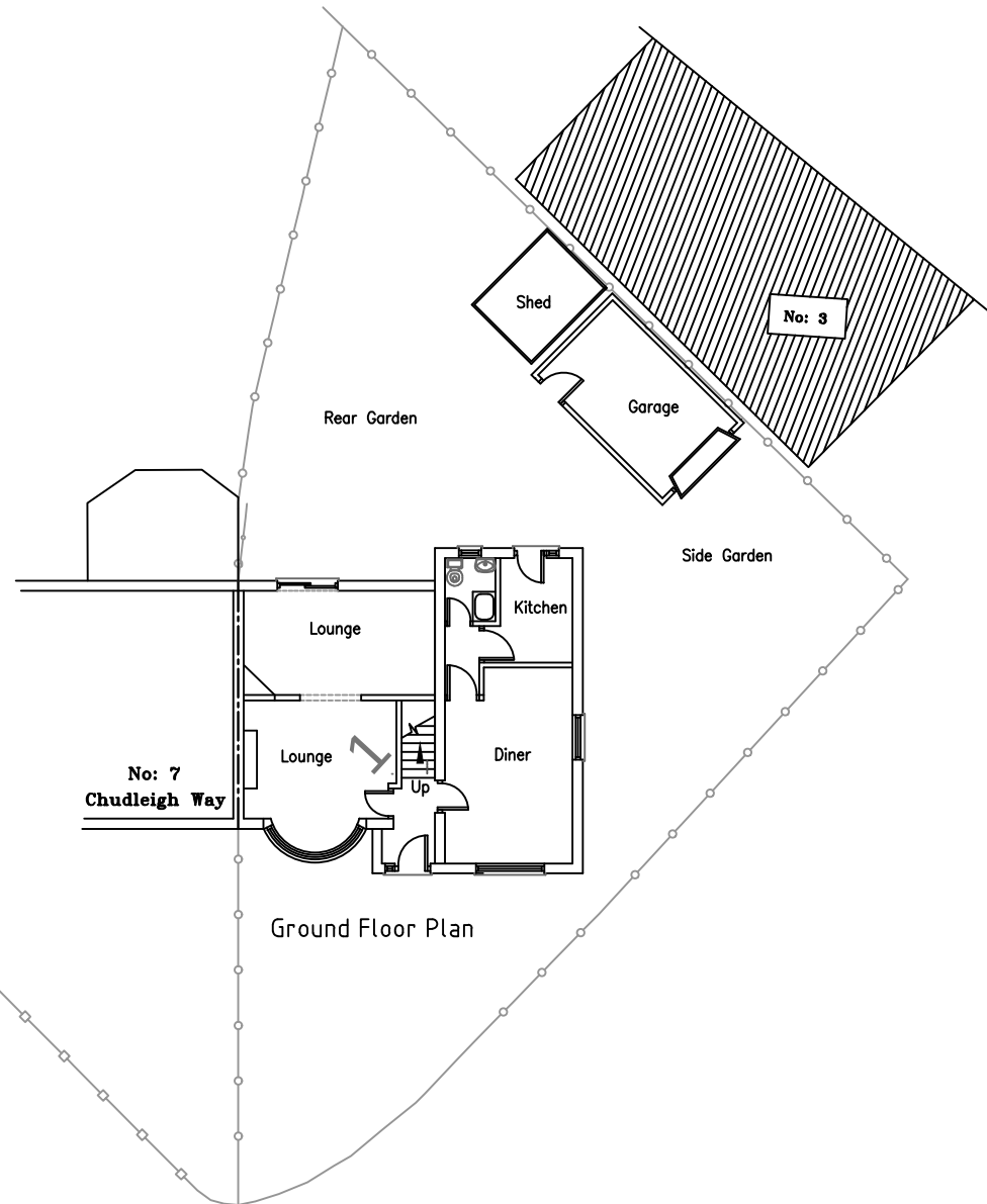
Existing Block Plan - 1:200 Ground Floor
