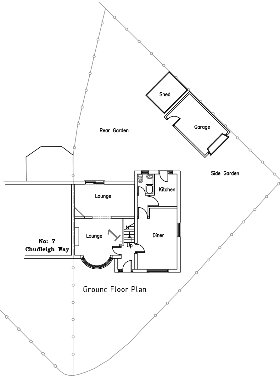
Existing Block Plan - 1:200 Ground Floor
