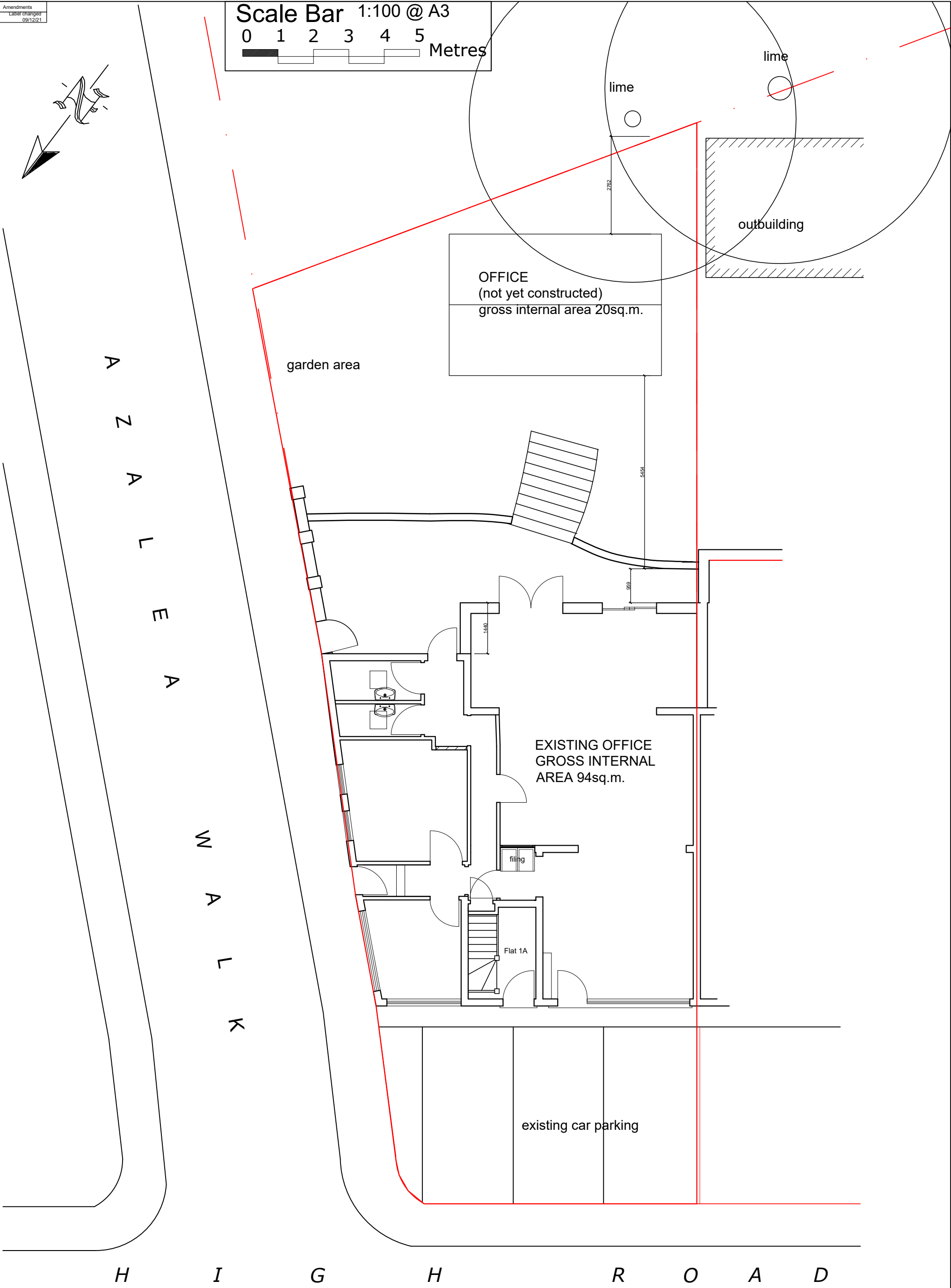
SITE PLAN
