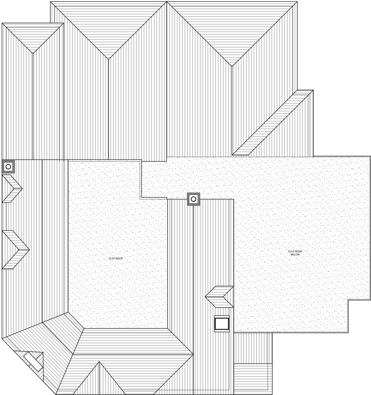
01- ROOF PLAN
