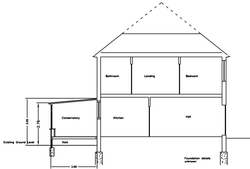
CROSS SECTION
