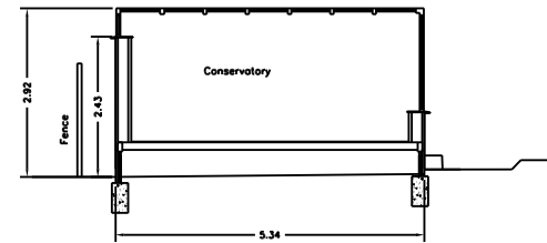
LONG SECTION
