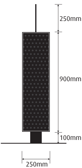
Side Elevation
