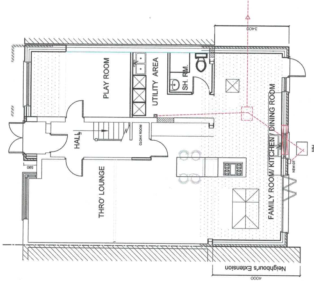
PROPOSED G/FLOOR
