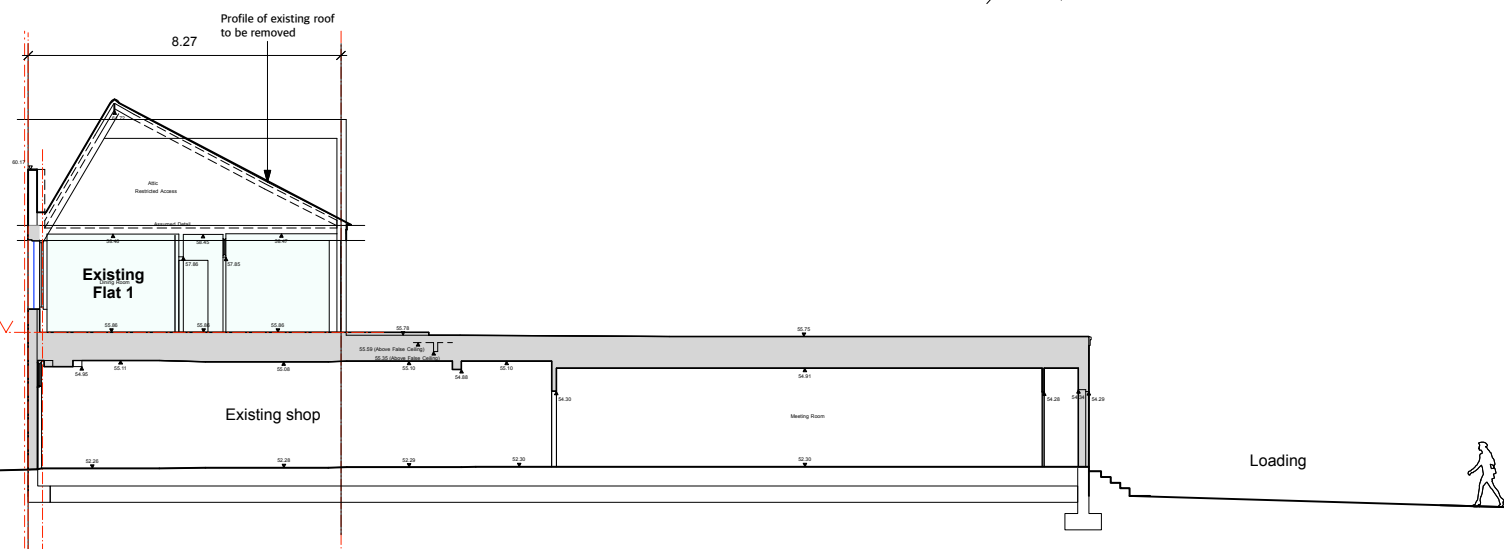
LONG SECTION LOOKING NORTH
