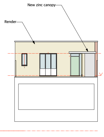
PODIUM [SW] ELEVATION AS PROPOSED
