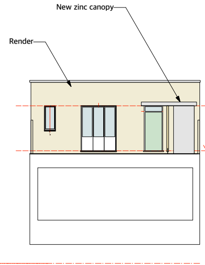
PODIUM [SW] ELEVATION AS PROPOSED
