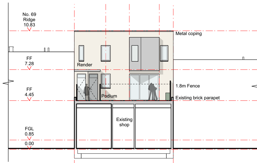
Section CC Rear (North East) Elevation of Front Building
