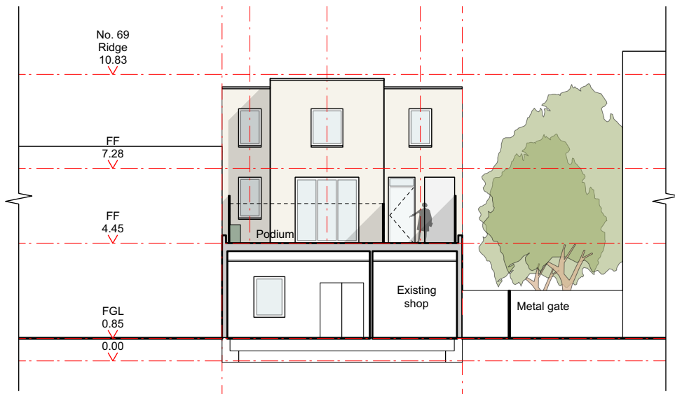
Section BB Internal South West Elevation of Rear Building
