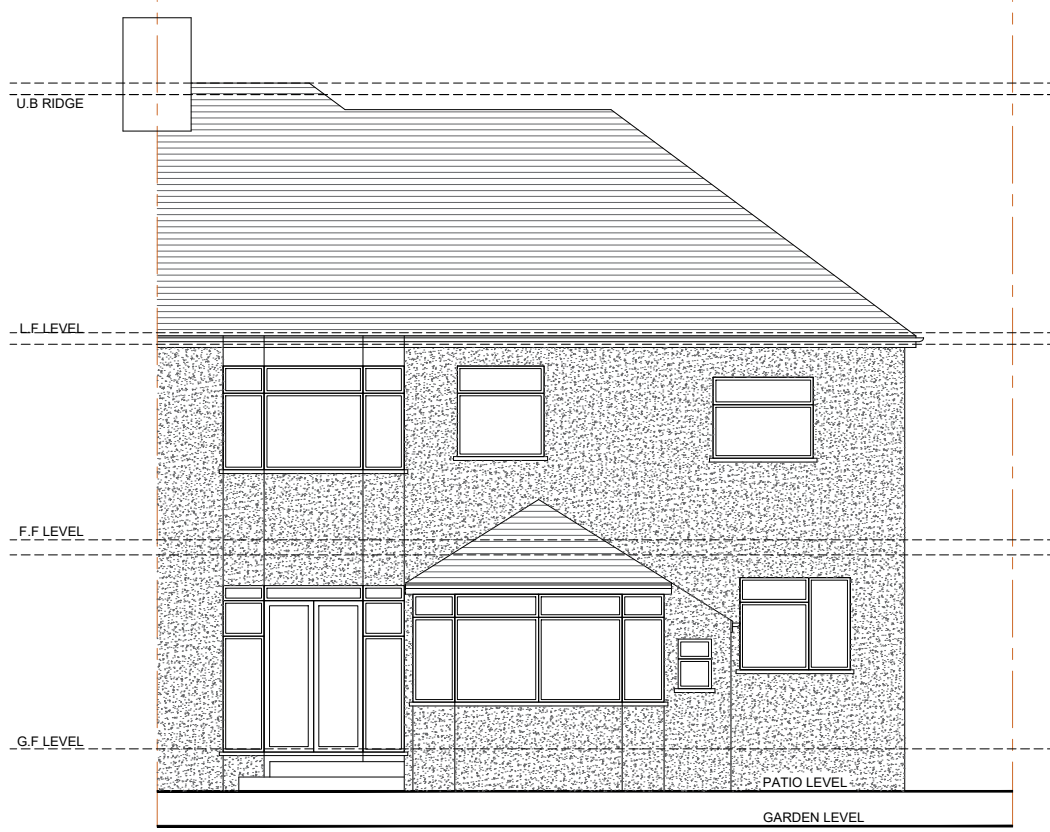
PRE EXISTING REAR ELEVATION
