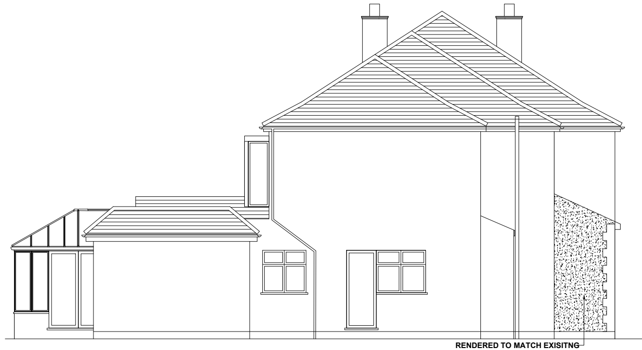
PROPOSED LEFT ELEVATION
