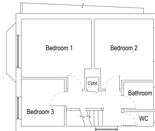
First Floor Existing
