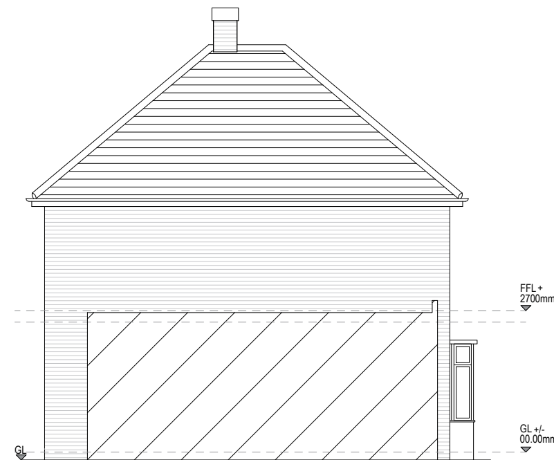
Side (W) Elevation Existing
