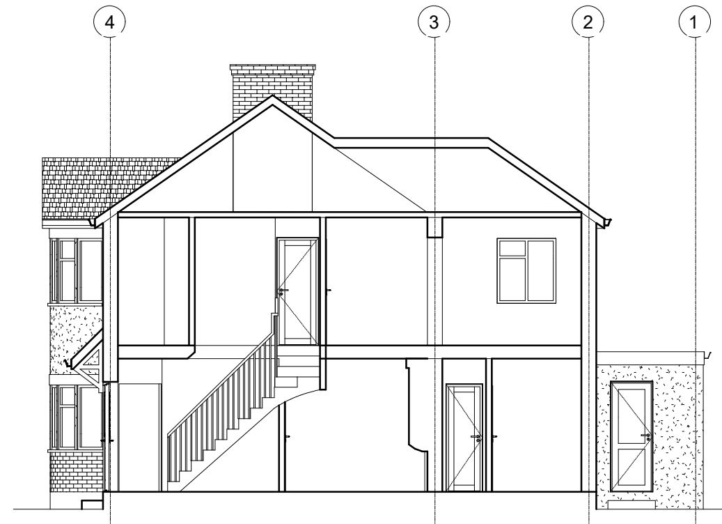
EXISTING SECTION
