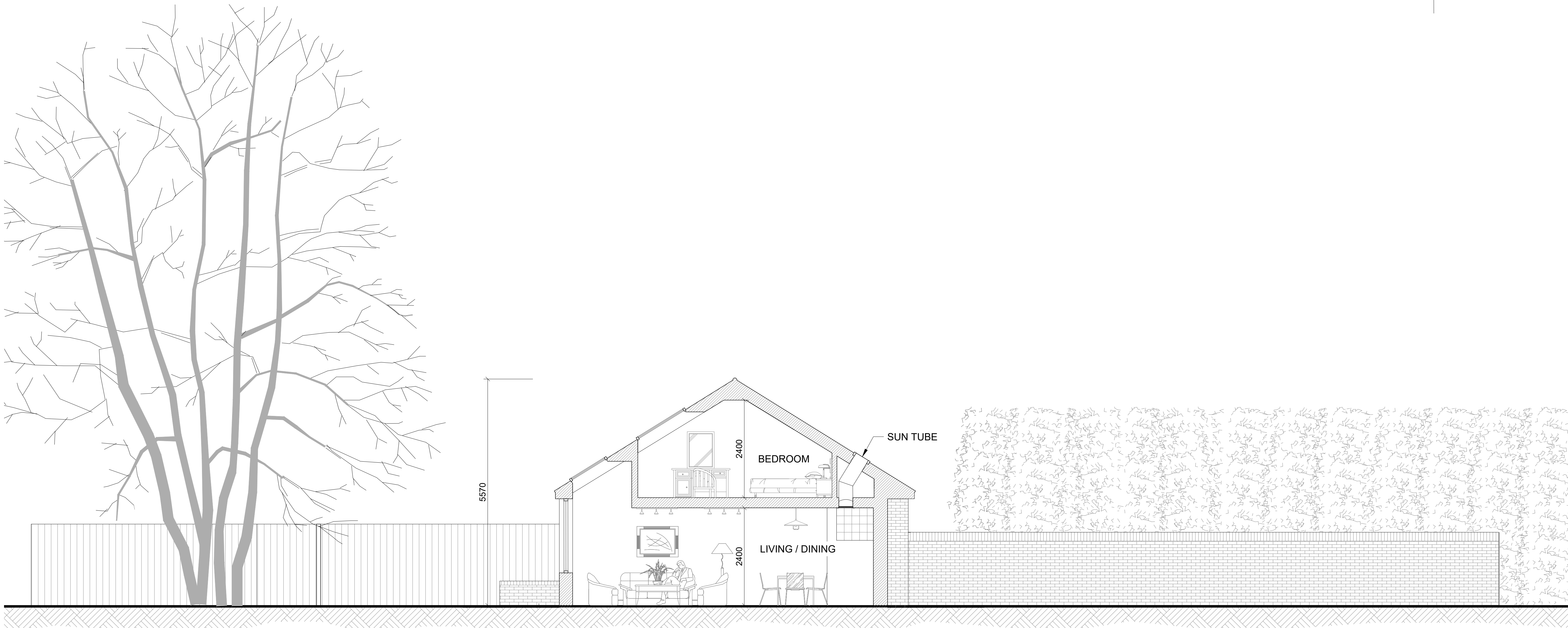
SECTION B-B
