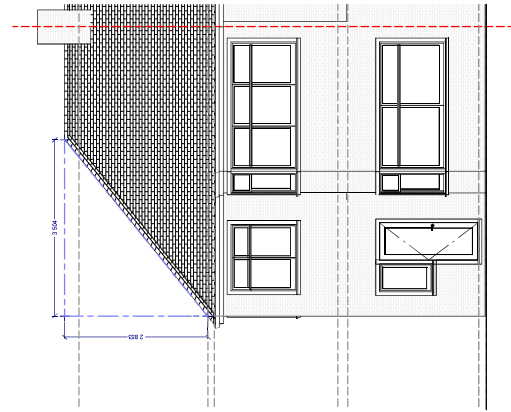
EXISTING FRONT (1:100)
