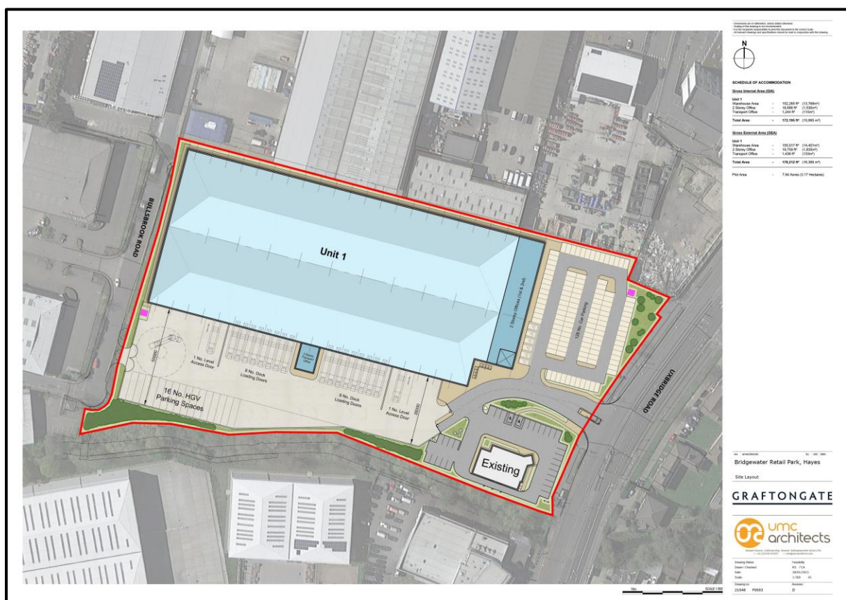
Figure 2.2: Layout of Proposed Development
