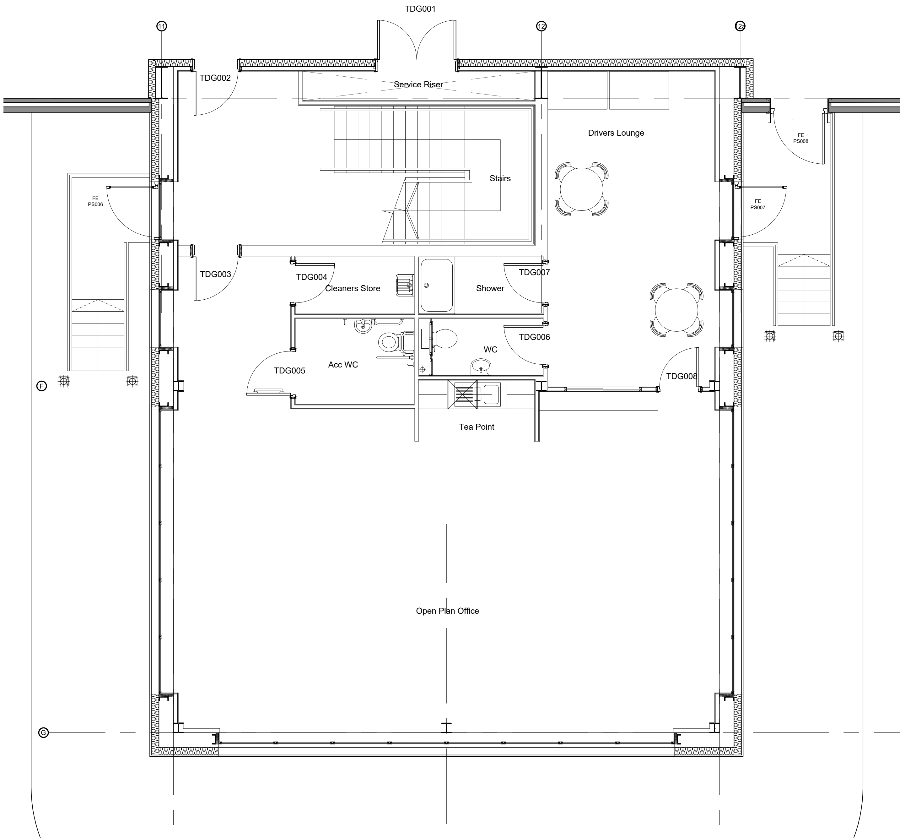
Proposed Transport Office Ground Floor Scale 1:50
