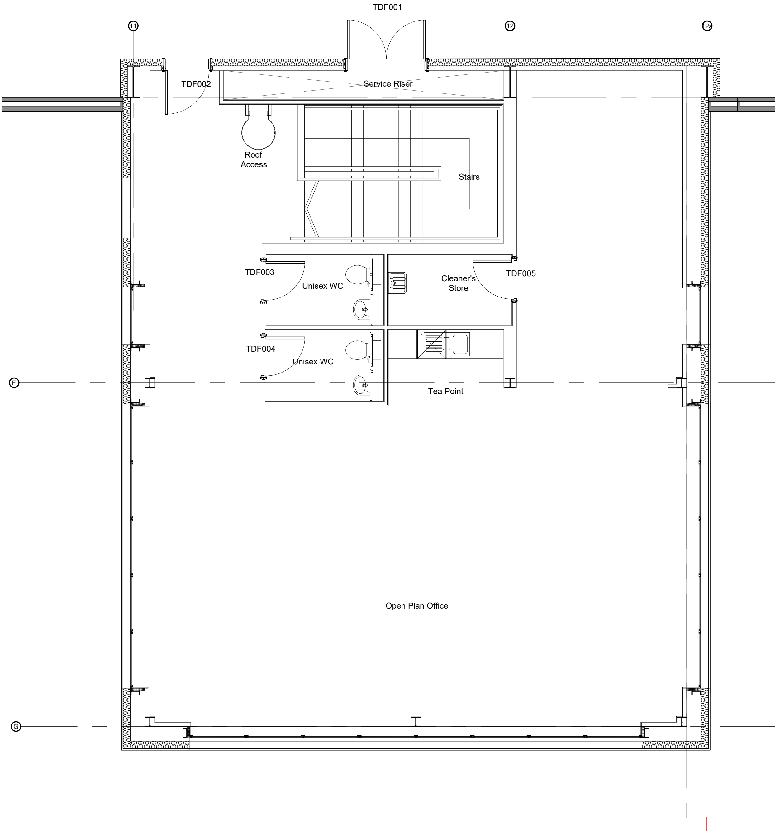
Proposed Transport Office First Floor Scale 1:50
