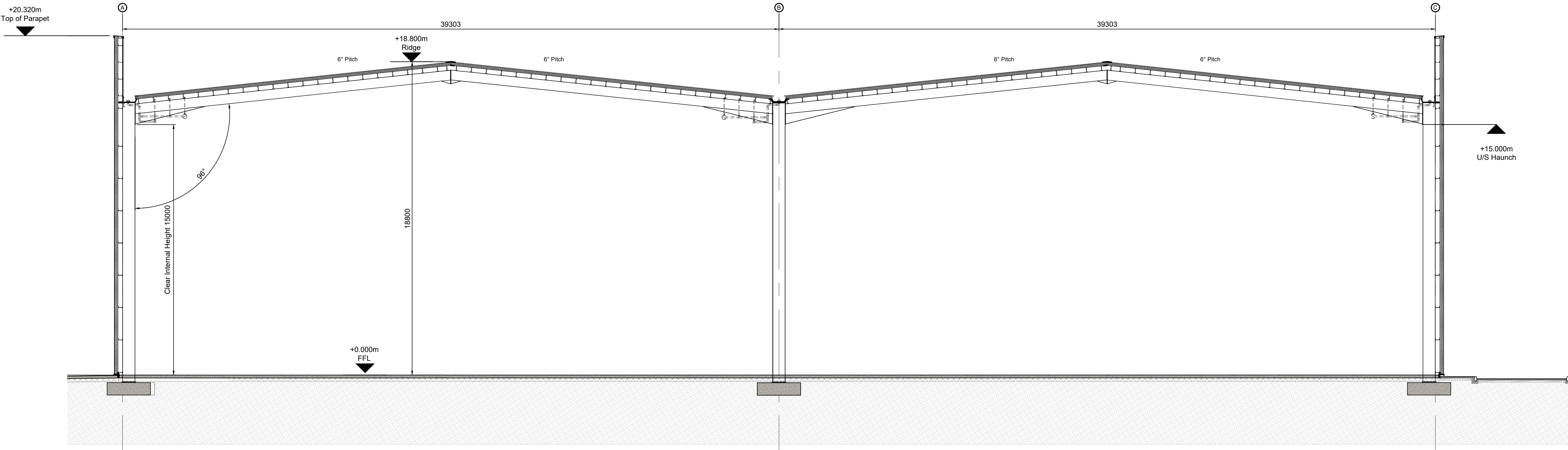
Proposed Section Scale 1:125
