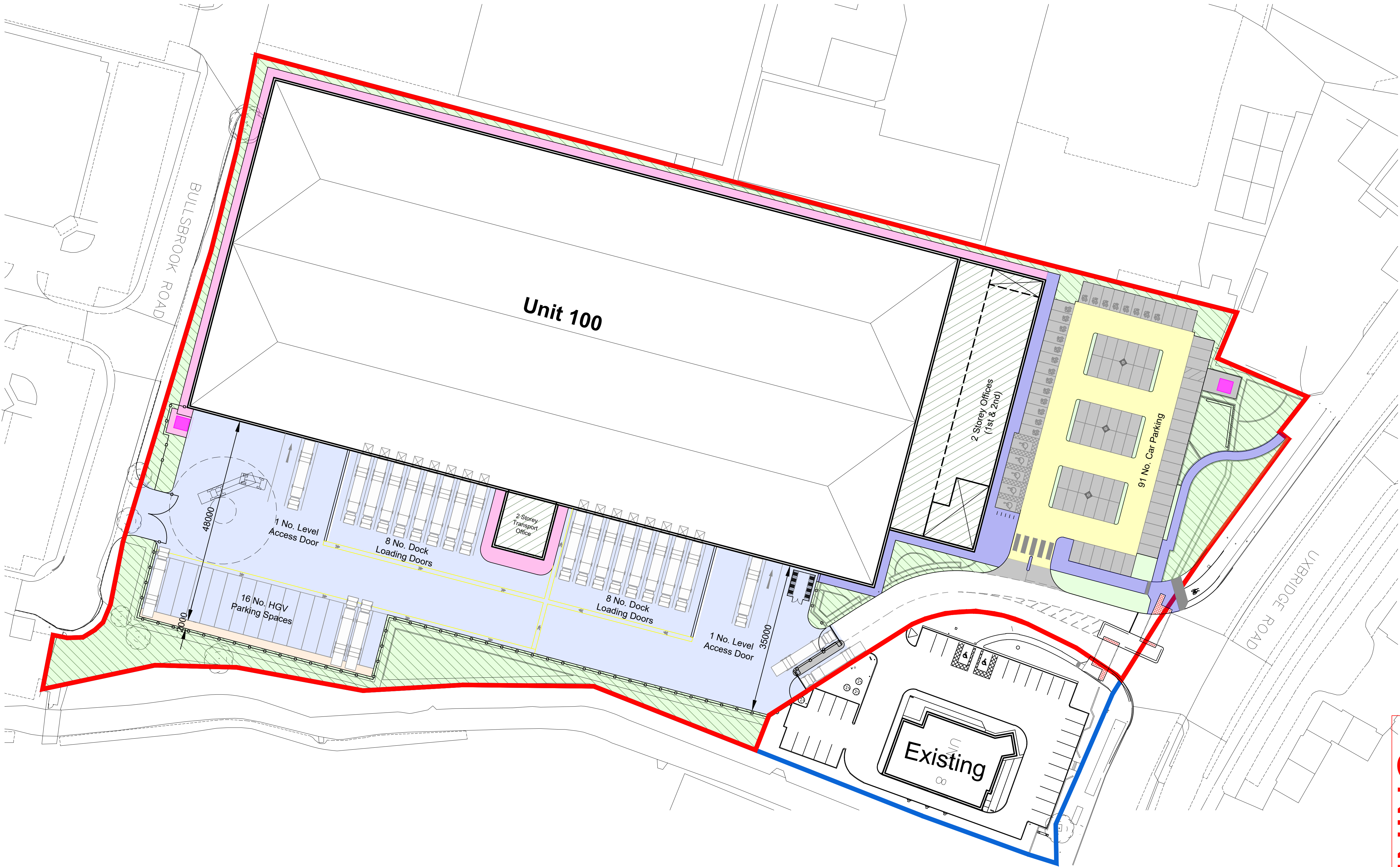
Proposed External Surfaces Plan Scale 1:500
