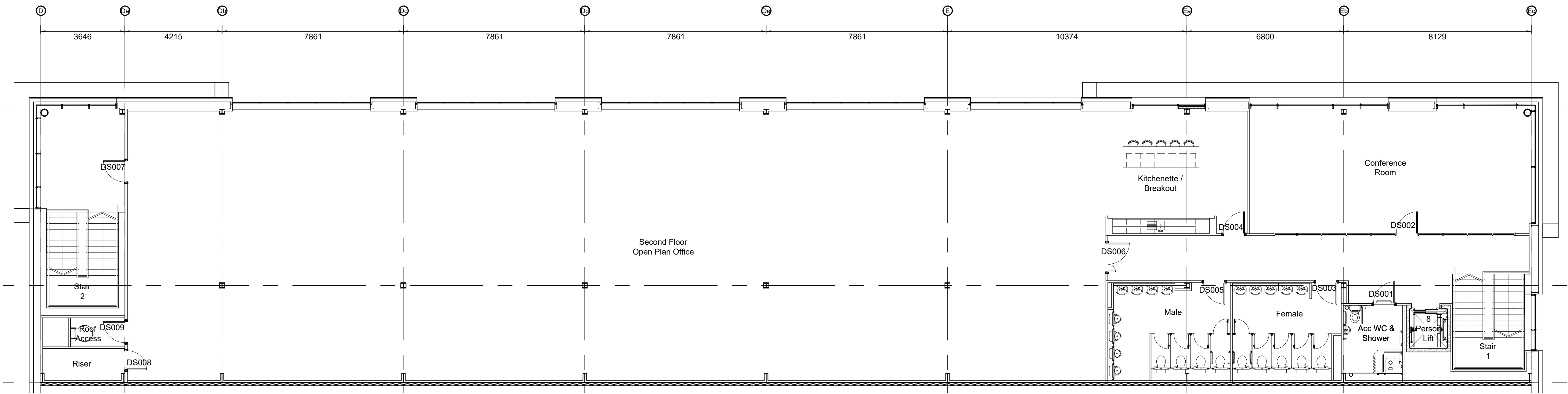
Second Floor Main Office Layout Scale 1:100
