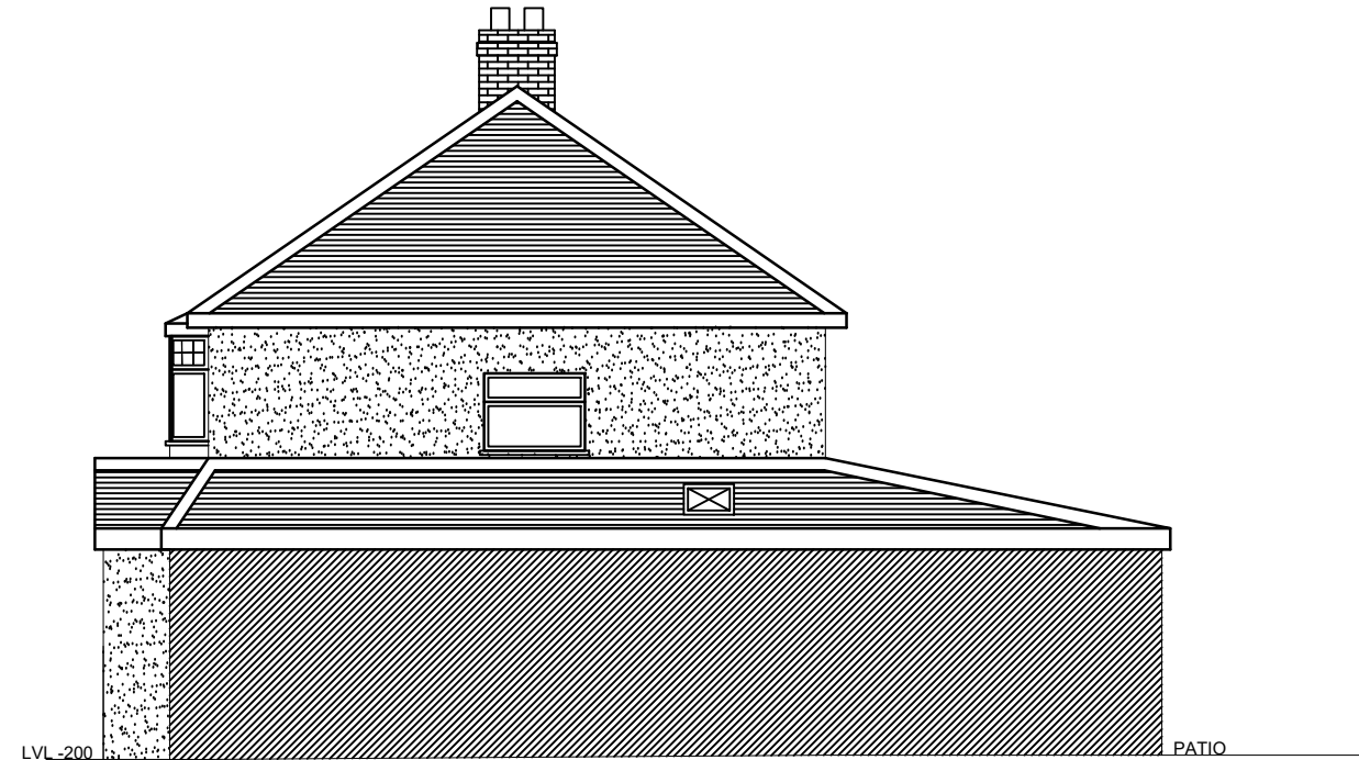
SIDE ELEVATION PROPOSED (AS VIEWED FROM NO:59)
