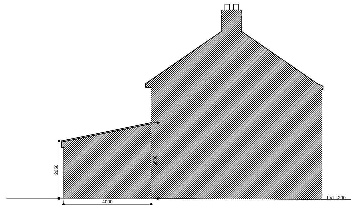
SIDE ELEVATION PROPOSED (AS VIEWED FROM NO:55)
