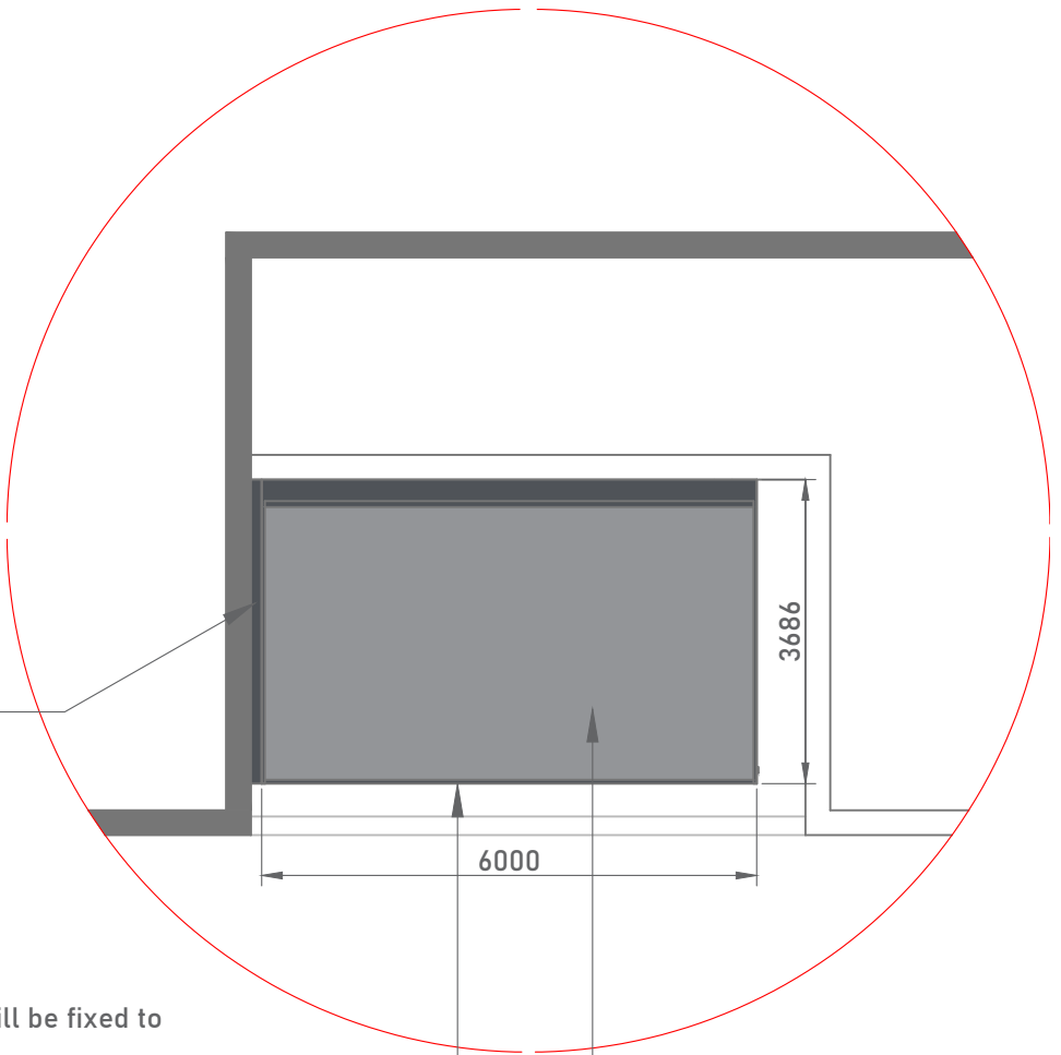
UPPER GROUND FLOOR PLAN
