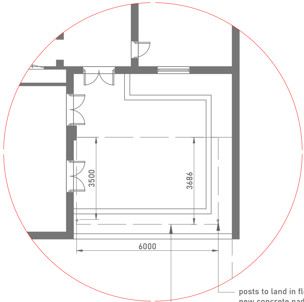
LOWER GROUND FLOOR PLAN
