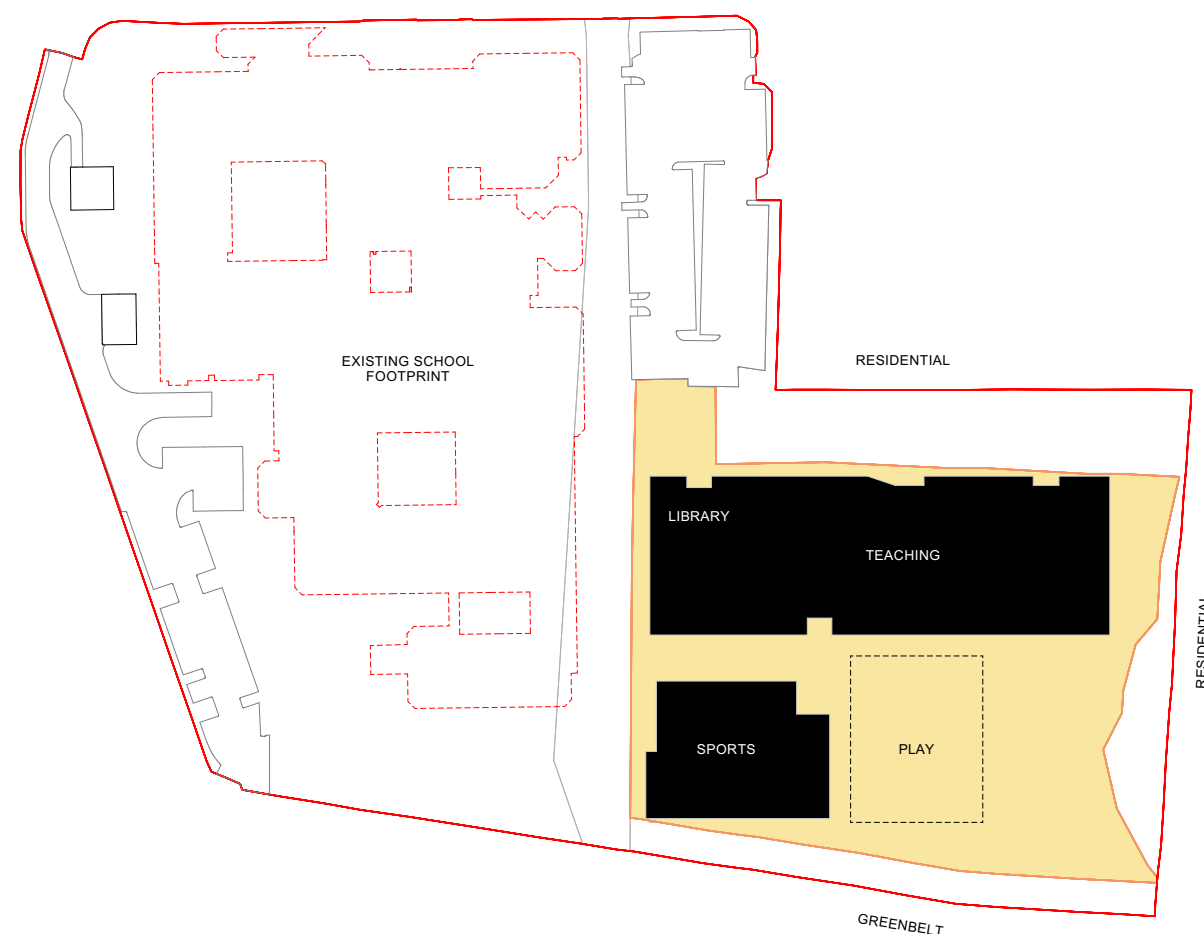
Site Study - Sports Building West
