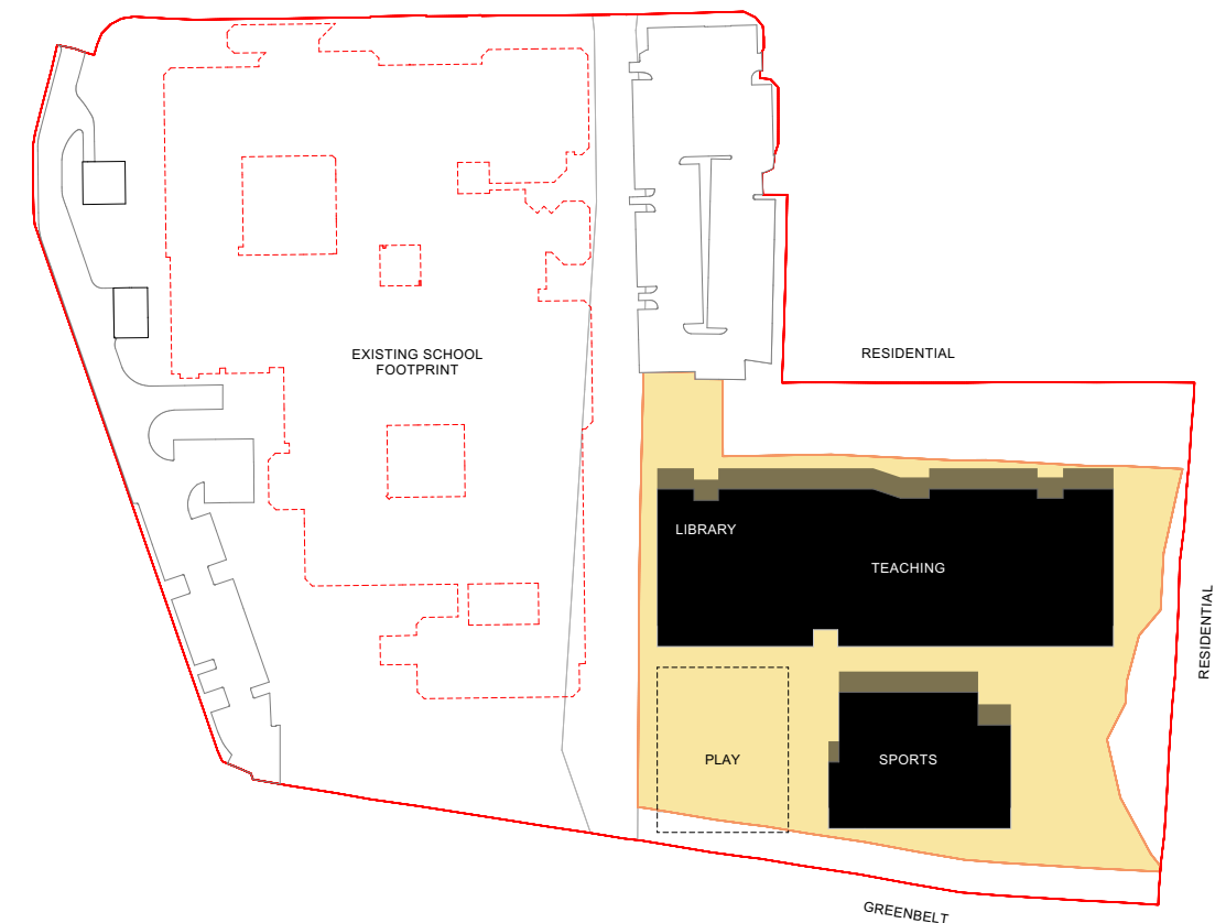
Illustrative Site Plan - Showing buildings moved 5m south
