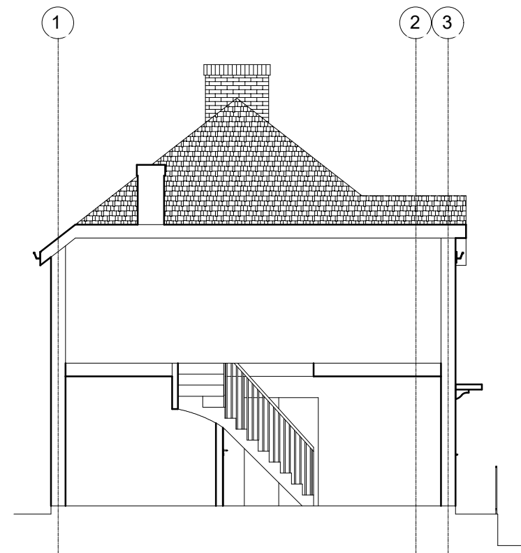
EXISTING SECTION
