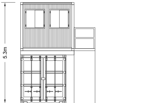
Side Elevation of Container and site Office
