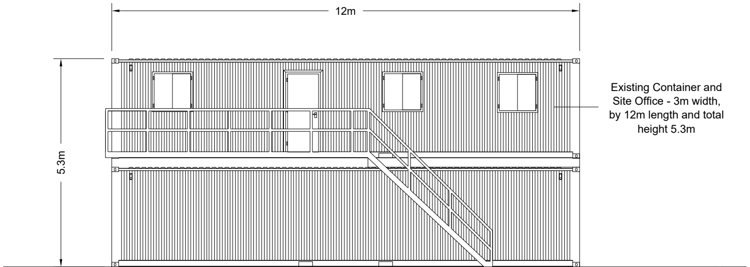
Front Elevation of Container and site Office
