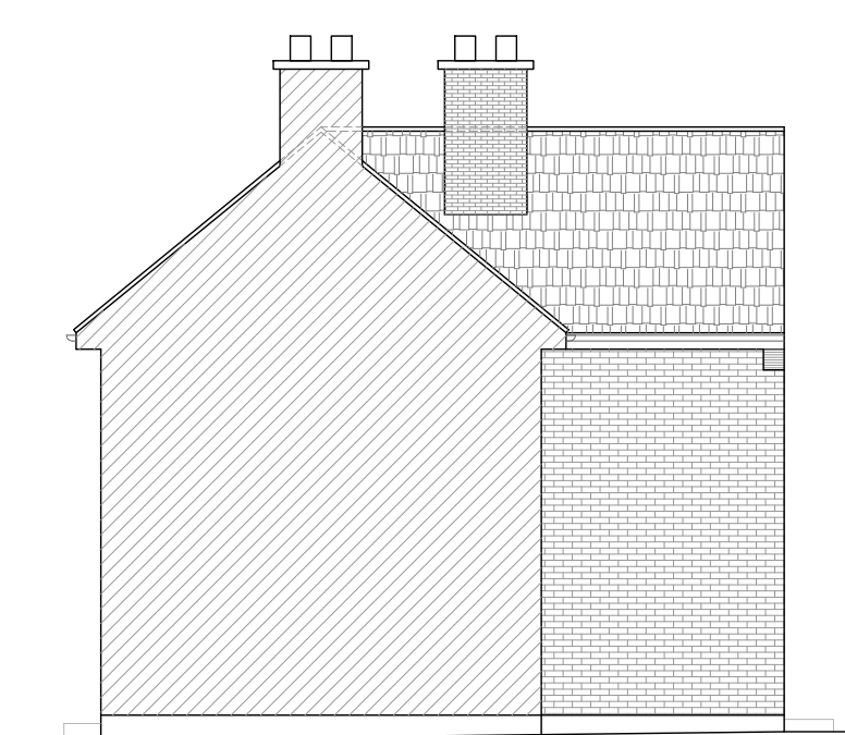
EXISTING SIDE ELEVATION-2
