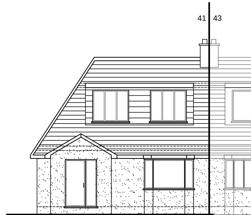
FRONT ELEVATION PROPOSED
