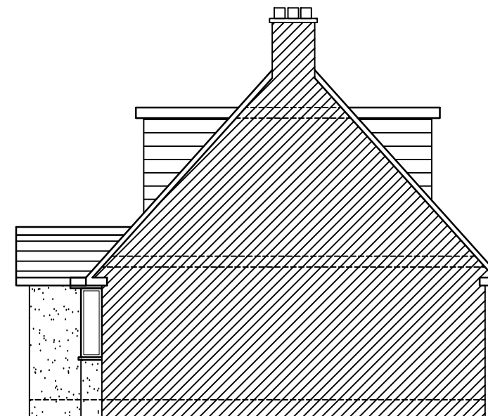
SIDE ELEVATION PROPOSED (PARTY WALL SIDE)
